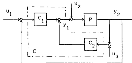
proper, D must be one because it is the constant term of (1 + aG)^{-1}(1 + (a - 1)G) . Therefore, the least upper bound of \{\operatorname{Re} \lambda; \lambda \in \sigma(A)\} is no less than zero. Hence, again by Hale [11, Corollary 1.7.1], the closed-loop system cannot be exponentially stable. ■
