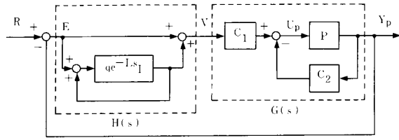
Fig. 8. Modified repetitive control system with two degrees of freedom.
