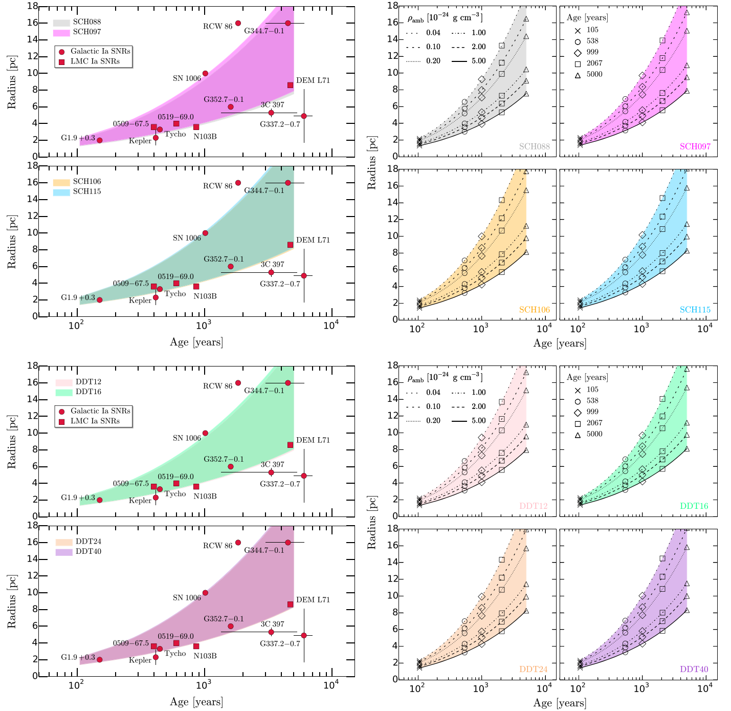
Figure 12. Forward shock radius vs. expansion age for the Type Ia SNRs in our sample. The shaded regions correspond to the models shown in Figures 9, 10, and 11.
