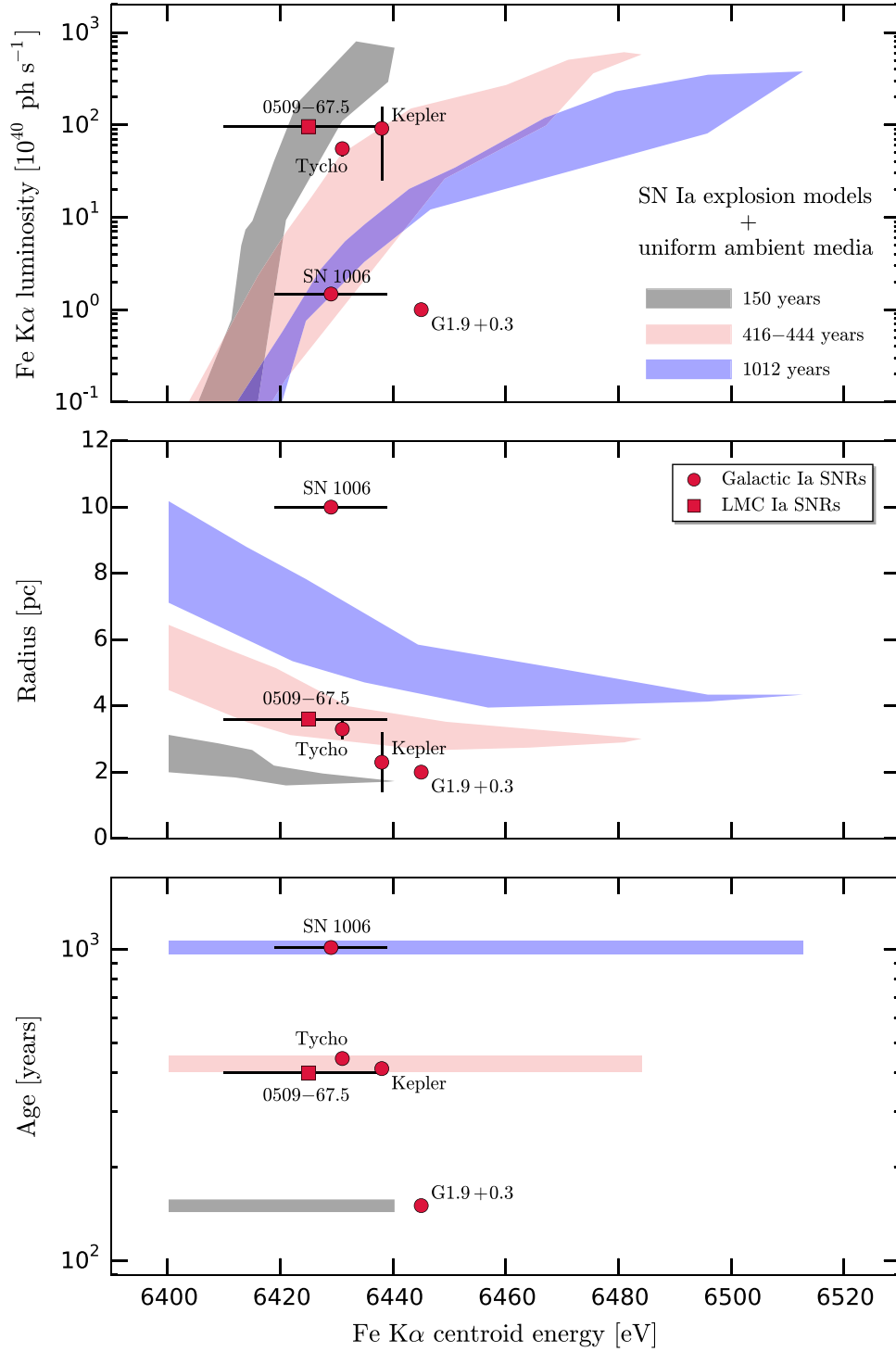
Figure 14. Fe K\alpha luminosity, radius, and expansion age as a function of the Fe K\alpha centroid energy for G1.9+0.3, 0509–67.5, Kepler , Tycho, and SN 1006. The shaded regions depict the predictions from our theoretical M_{\text{Ch}} and sub- M_{\text{Ch}} models with uniform ISM densities for different expansion ages: 150 (black), 416–444 (light coral), and 1012 (blue) years.
