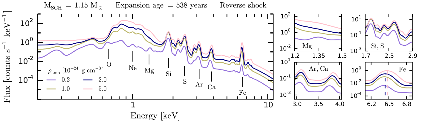
Figure 5. Integrated RS synthetic spectra normalized to D = 10 kpc for model SCH115, for the four highest ambient densities ( \rho_{0p2} , \rho_{1p0} , \rho_{2p0} , \rho_{5p0} ) and a fixed expansion age of 538 years. The zoomed boxes are identical to those of Figure 4.
