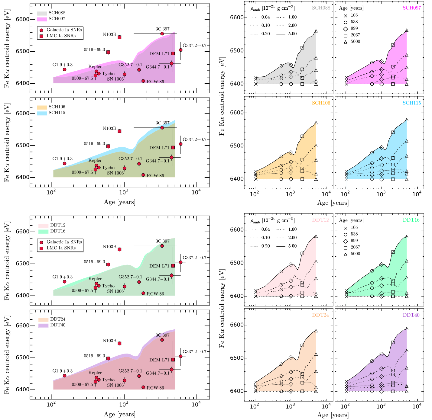
Figure 11. Fe K \alpha centroid energy vs. expansion age for the Type Ia SNRs in our sample. The shaded regions correspond to the models shown in Figures 9 and 10.
