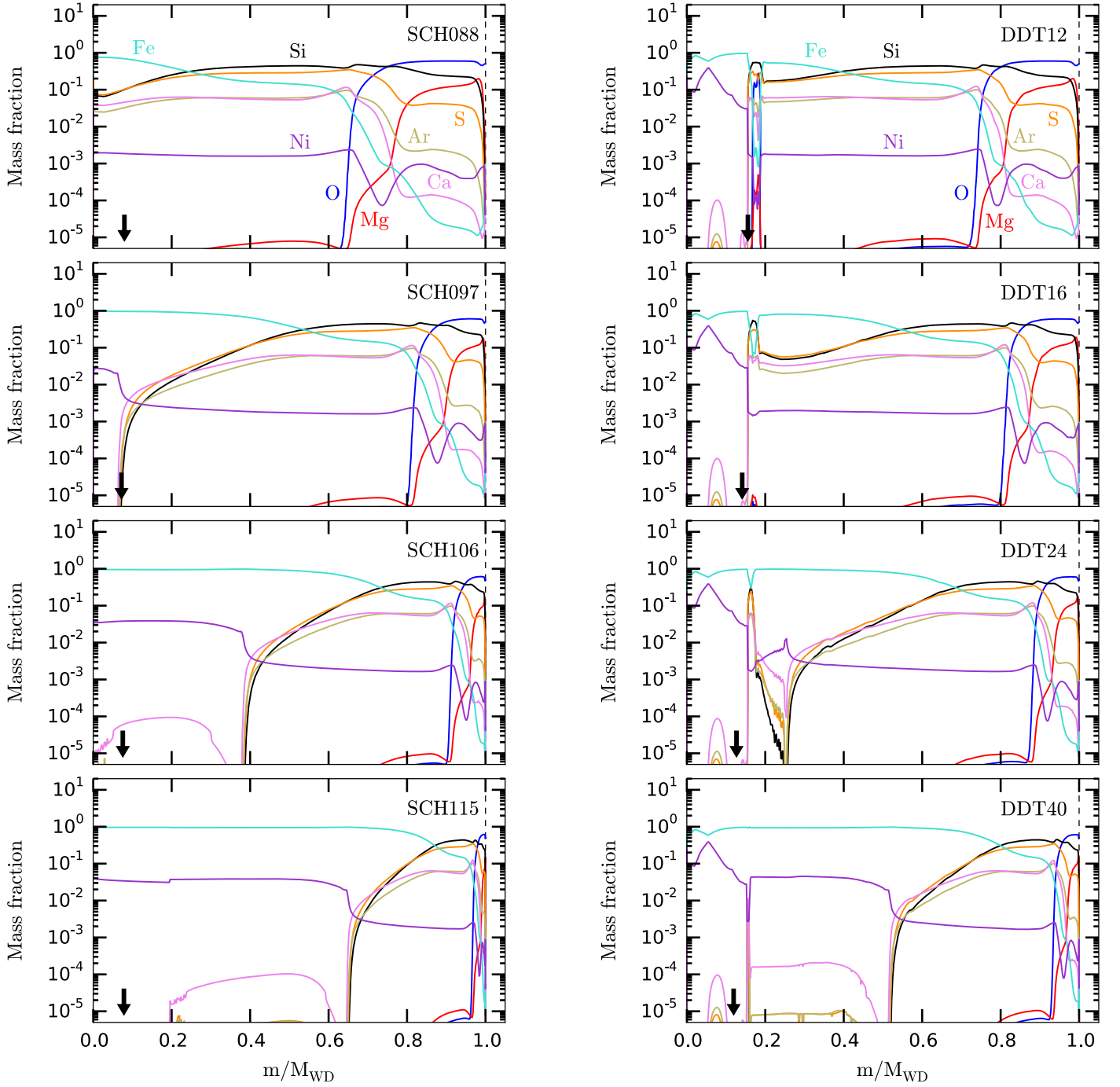
Figure 1. Chemical composition for our SN Ia models listed in Table 1. The vertical, dashed lines indicate the outer surface of each ejecta model. The arrows depict the locations of the RS at 538 years for \rho_{\text{amb}} = 2 \times 10^{-24} \text{ g cm}^{-3} (see the discussion in Section 2.3).
