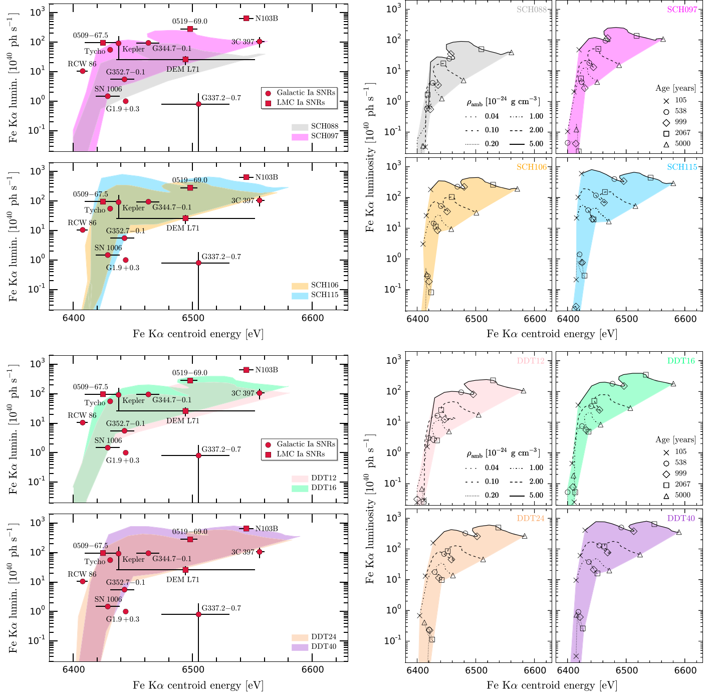
Figure 9. Left: centroid energies and line luminosities of Fe K \alpha emission from various Type Ia SNRs in our Galaxy (circles) and the LMC (squares). The shaded regions depict the Fe K \alpha centroids and luminosities predicted by our theoretical sub- M_{\text{Ch}} and M_{\text{Ch}} models with various uniform ISM densities (SCH088: gray; SCH097: magenta; SCH106: orange; SCH115: blue; DDT12: pink; DDT16: green; DDT24: light brown; DDT40: purple). Right: individual tracks for each model. The L_{\text{FeK}\alpha} - E_{\text{FeK}\alpha} tracks corresponding to the two lowest ambient densities ( \rho_{0p04} , \rho_{0p1} ) do not appear in the plots because their L_{\text{FeK}\alpha} values are considerably small.
