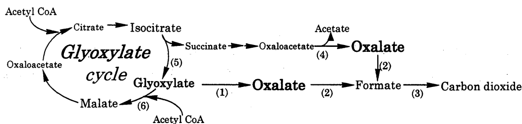
Fig. 2. Glyoxylate cycle and oxalate metabolism in white-rot fung. (1) Glyoxylate dehydrogenase, (2) Oxalate decarboxylase, (3) Formate dehydrogenase, (4) Oxaloacetase, (5) Isocitrate lyase, (6) Malate synthase.
