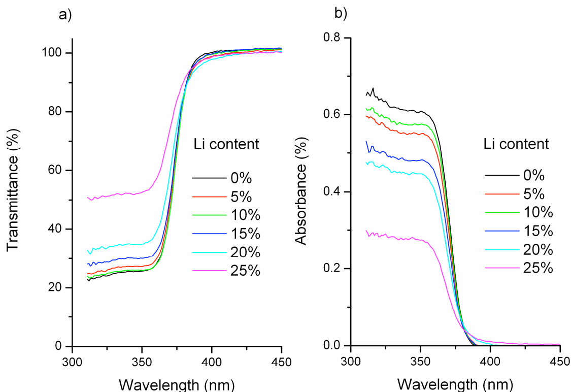
Fig. S5 Transmittances and absorbances of Li doped ZnO nanorods at various Li content coated on glass substrate.
