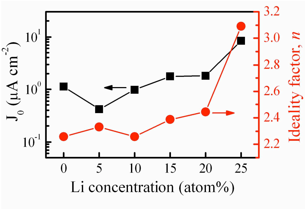
Reverse current density ( J_0 ) and ideality factor ( n ) of hybrid Zn1-xLixO nanorods/P3HT solar cells ( x = 0 - 0.25 ). 71x49mm (600 x 600 DPI)
