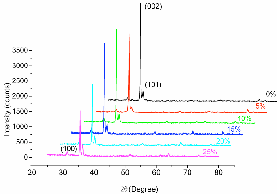
Fig. S2 The XRD patterns of \text{Zn}_{1-x}\text{Li}_x\text{O} nanorods.
