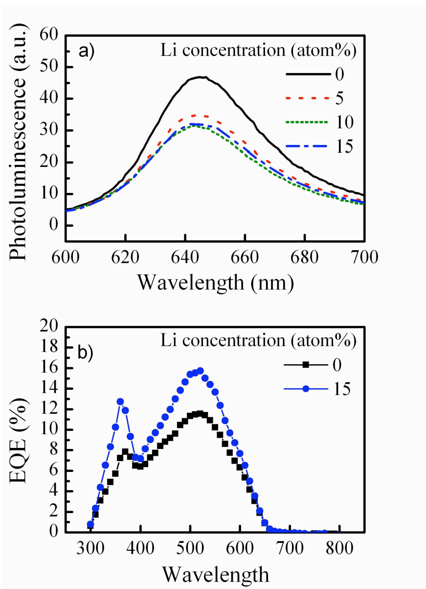
a) photoluminescence of hybrid Zn 1-x Li x O nanorods/P3HT films on glass substrates ( x = 0 - 0.15 ) and b) the EQE of hybrid Zn 1-x Li x O nanorods/P3HT solar cells ( x = 0, 0.15 ) 71x98mm (600 x 600 DPI)
