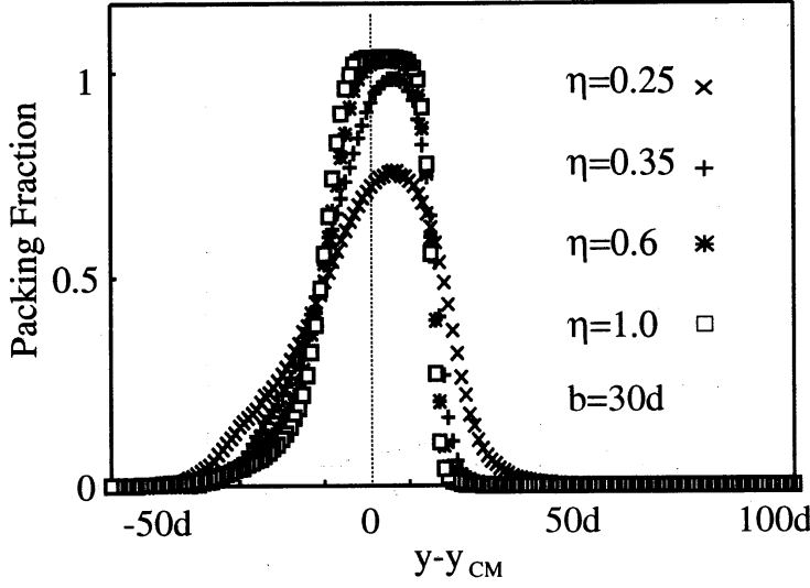
Fig. 3. Packing fraction profile for y direction respectively \eta = 0.25, 0.35, 0.6 , and 1.0 .
