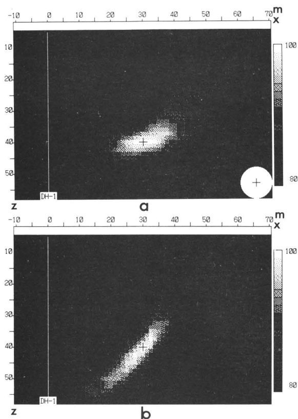
Fig. 8. Evaluation of solid array spacing and line effects in resistivity computerized sections obtained by the construction procedures. (a): Section in the case of Fig. 7a, (b): Section in the case of Fig. 7b.
