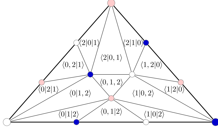
Figure 5: Standard chromatic subdivision of a 2-dimensional simplex, where the facets are labeled with ordered set partitions.
