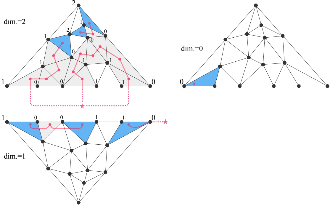
Figure 1: Graphs derived from Sperner labeling, for dimensions 2, 1, and 0
