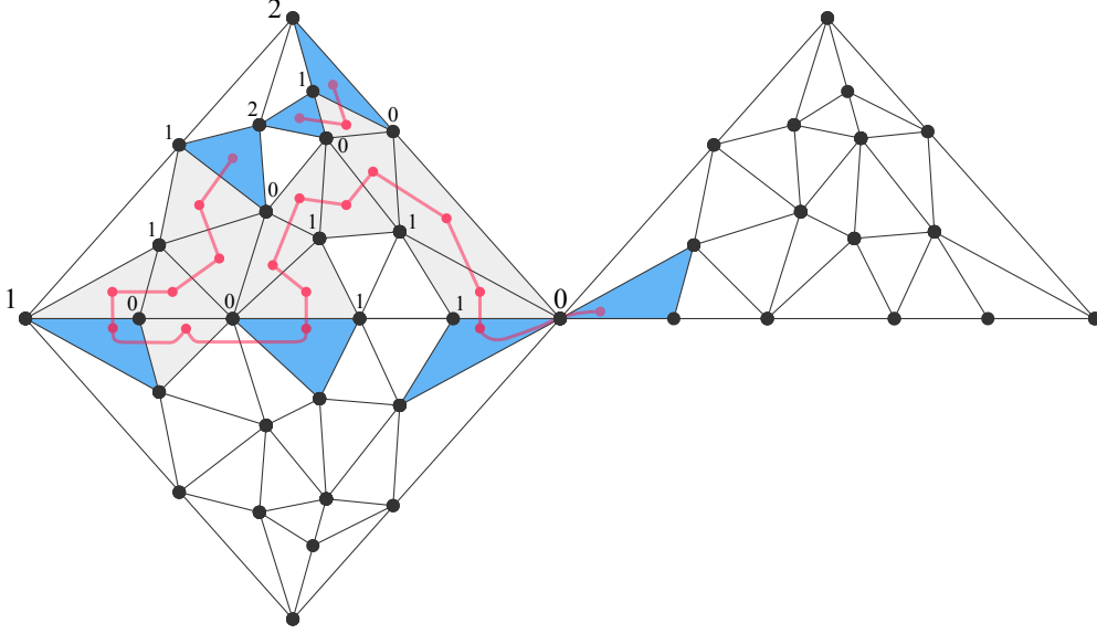
Figure 2: Unified graph of all the induction cases of dimensions 2, 1, and 0
