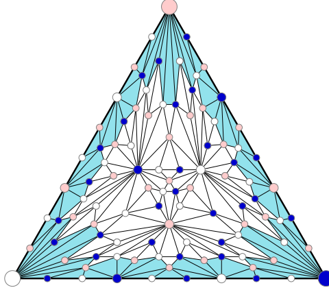
Figure 7: 2-concurrency model R2 for a 3-process system, a subcomplex of \mathcal{IS}^2 that consists of the shaded facets
