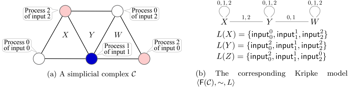
Figure 4: A topological model and its corresponding Kripke model for a 3 process system
