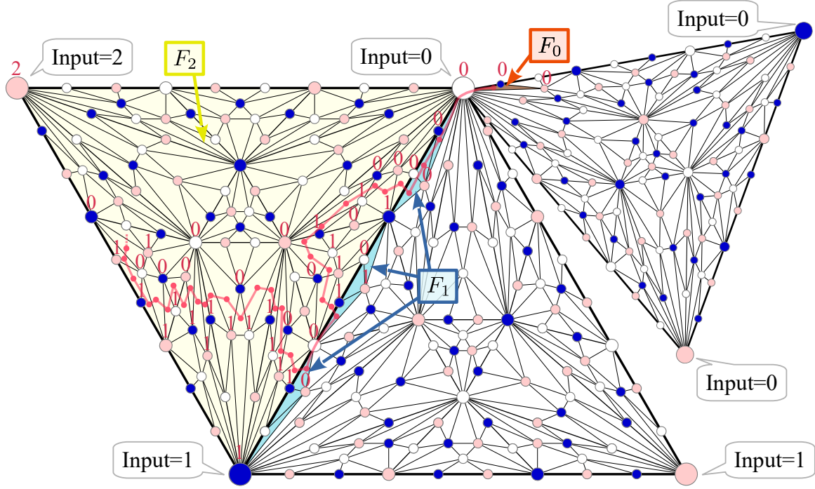
Figure 6: Collections of facets F_0 , F_1 , and F_2 that are contained in the product update model \mathcal{I}[\mathcal{IS}^2]_\delta . The numbers on the vertexes indicate the output values decided by \delta . The solid red lines indicate an (incomplete) graph path over the facets that are connected by either of the relations \frown_{\{0\}} and \frown_{\{0,1\}} .
