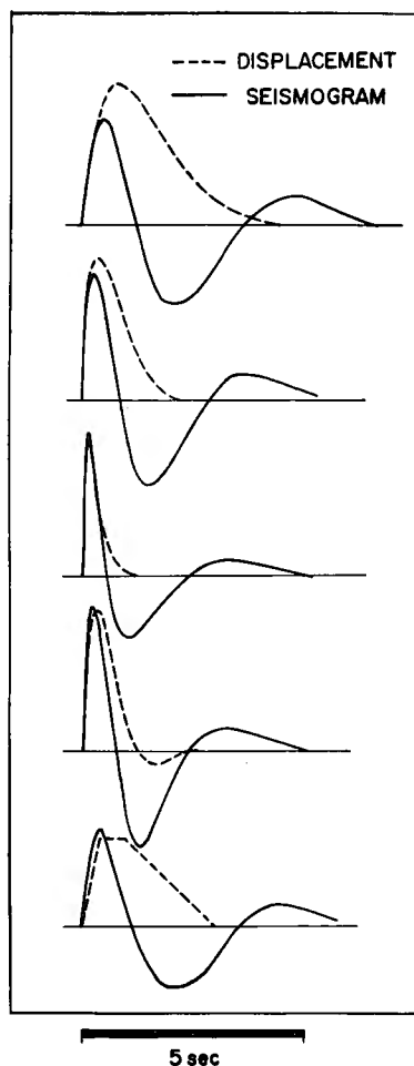
Fig. 4. Assumed ground motions and corresponding wavelets to be recorded by the Wiechert-type seismograph.
