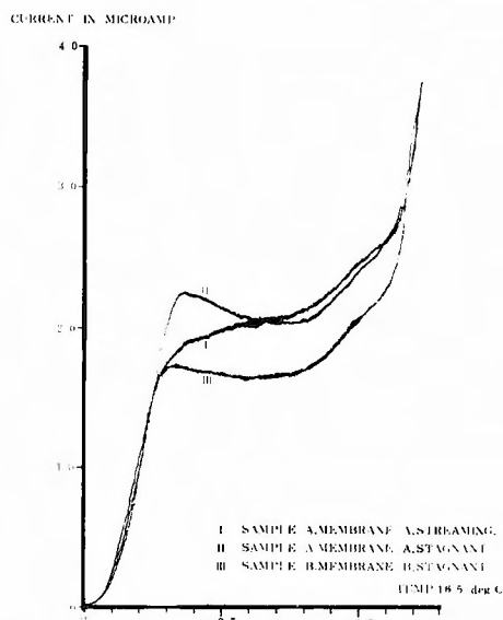
Fig. 4. The Current-Voltage Curves of Oxygen recorded polarographically with the use of Clark Oxygen Electrode in the physiological saline solutions under the various conditions and at the stable temperature of 16.5 degrees C.
