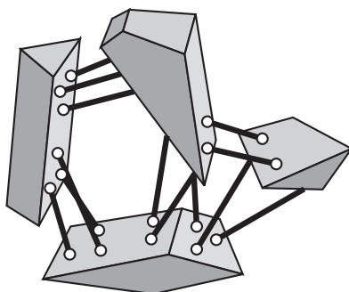
FIG. 4. A finite body-and-bar framework in three dimensions.
