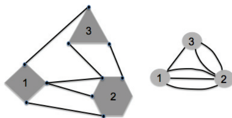
FIG. 3. A finite, minimally rigid body-and-bar framework in two dimensions, with three bodies and six bars, and its associated multigraph.
