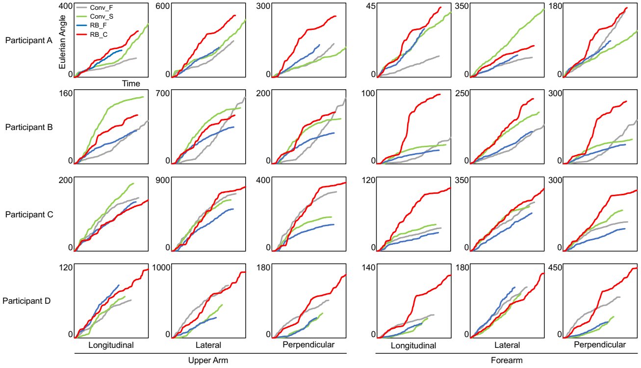
Fig. 5. Line charts showing the over time accumulated rotation of (left) the upper arm and (right) the forearm in Eulerian angle ( ^{\circ} ). From left to right is the rotation at the three axis, Longitudinal, Lateral, Perpendicular respectively, of world Cartesian coordinate. In the chart, each line stands for each pegboard condition (Conv_F: conventional pegboard flat; Conv_S: conventional pegboard slant; RB_F: RehaBricks flat; RB_C: RehaBricks convex). In short, this figure is aimed to quantitatively show how much the upper arm and the forearm have rotated in total throughout the trial.
