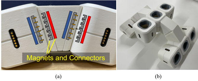
Fig. 3. Pictures showing (a) the curved piece which has magnets and spring-loaded connectors embedded, and (b) a convexly assembled board pattern using four curved pieces.
