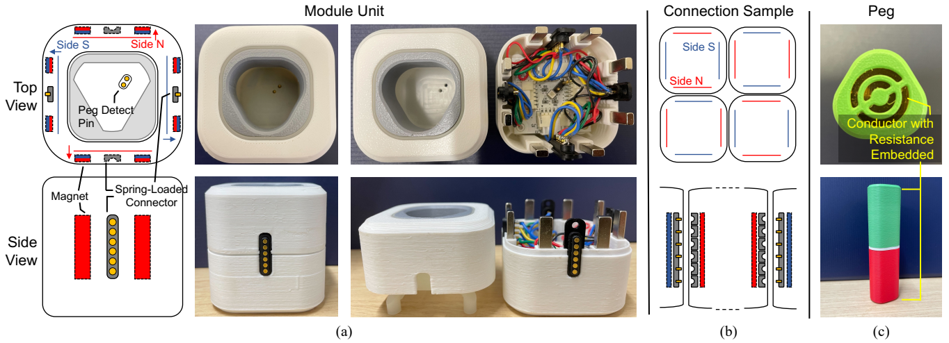
Fig. 2. Pictures and illustrated descriptions of the components and concept of our RehaBricks system. (a) Key features of the basic module unit. (b) Male/female spring-loaded connectors and magnets of opposite polarities are assigned to each side for geometric and electrical connection. (c) The peg has a halo-like conductor and resistance embedded in each side, allowing for detection of various pegs regardless of the shape of the peg hole and the orientation of the peg. We are not showing the specific measurements of each unit as the size is theoretically flexible, only limited by the size of the embedded circuit board.
