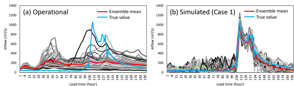
Fig. 2 Ensemble inflow prediction for Flood Event A: (a) operational prediction, (b) synthetically generated prediction (Case 1).
