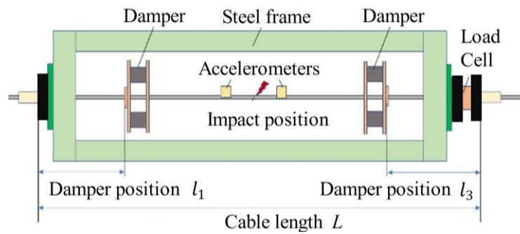
(a) Schematic diagram of test specimen, impact position, and measurement locations
