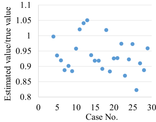
Fig. 6 Ratio of estimated tension to true tension using damper design formula (Eq.(33))
