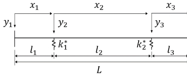
Fig. 1 Analytical model of a cable with two dampers
