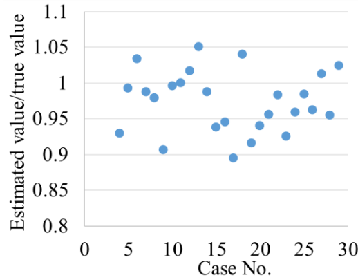
Fig. 7 Ratio of estimated tension to true tension using refined damper formula (Eq.(34))
