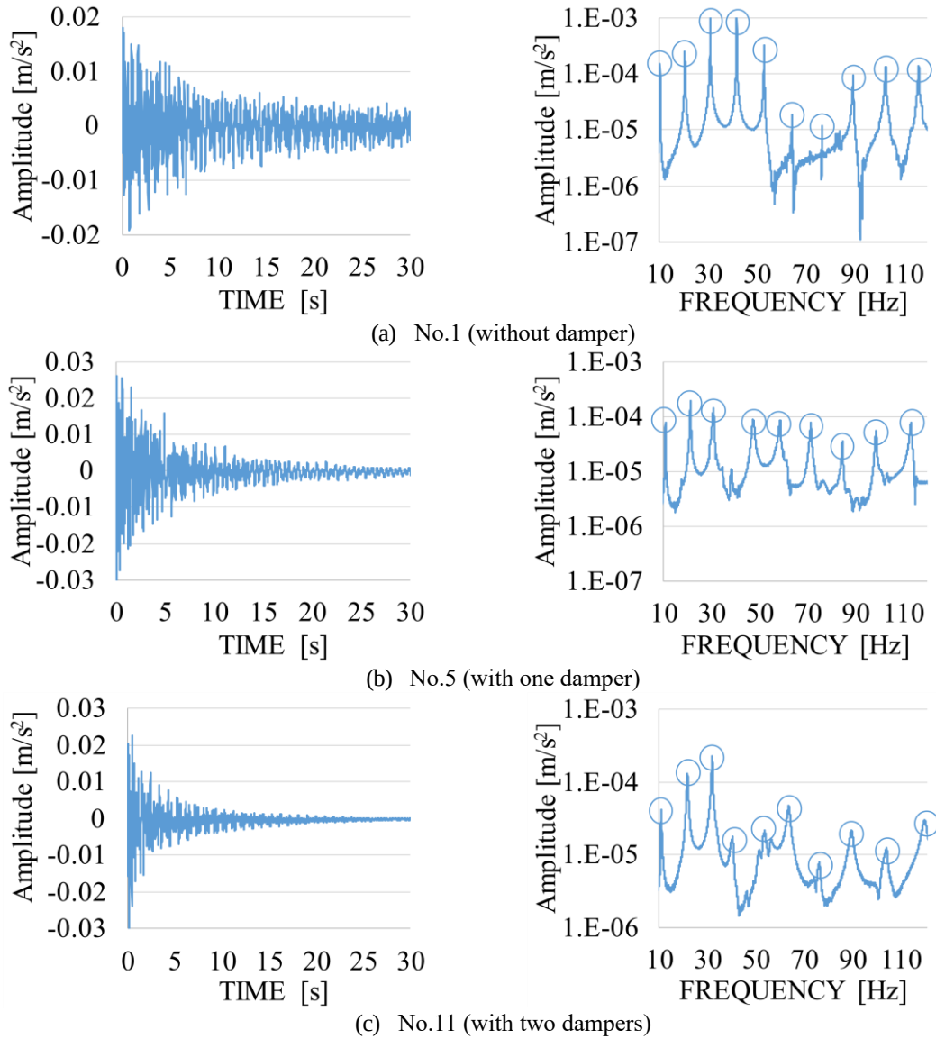
Fig. 5 Acceleration time history and Fourier spectrum for cases with approximately 20 kN tension
