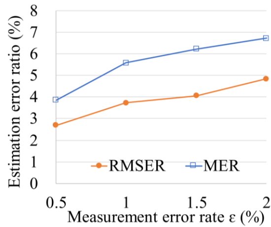
Fig. 3 Relationship between measurement error rate in natural frequency and tension estimation error ratio
