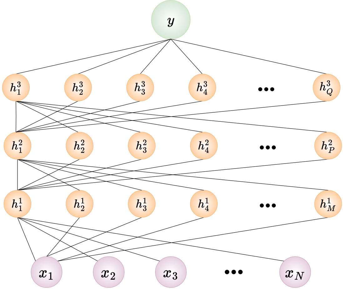
Figure 3.3: A multilayer feed forward neural network with inputs x_1, x_2, \dots, x_N and a single output y . There are 3 hidden layers in this network. At each neuron of the hidden layer Eq. (3.33) is carried out. The simplest form of this neural network will have only a single hidden layer.
