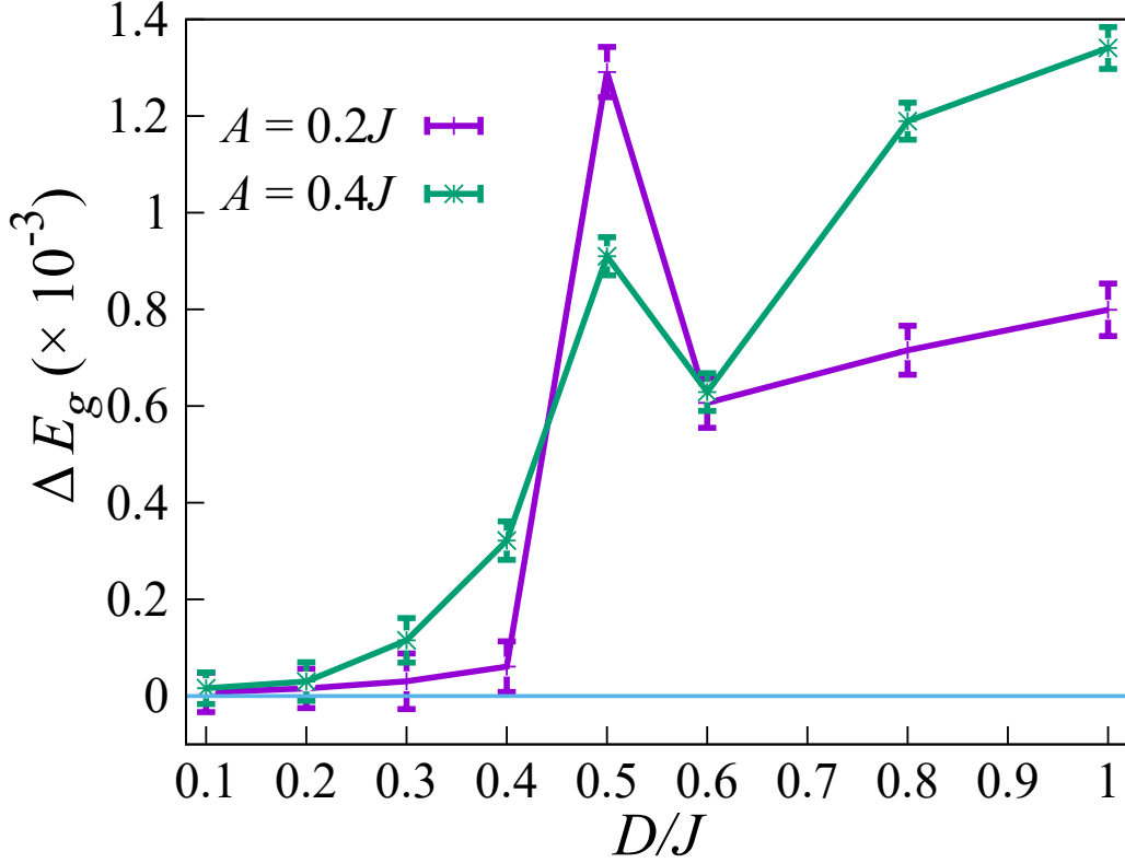
Figure 4.5: Relative energy gap \Delta E_g between the ground state and the first excited state found by the NQS method over DMI at A = 0.2J and A = 0.4J [21].
