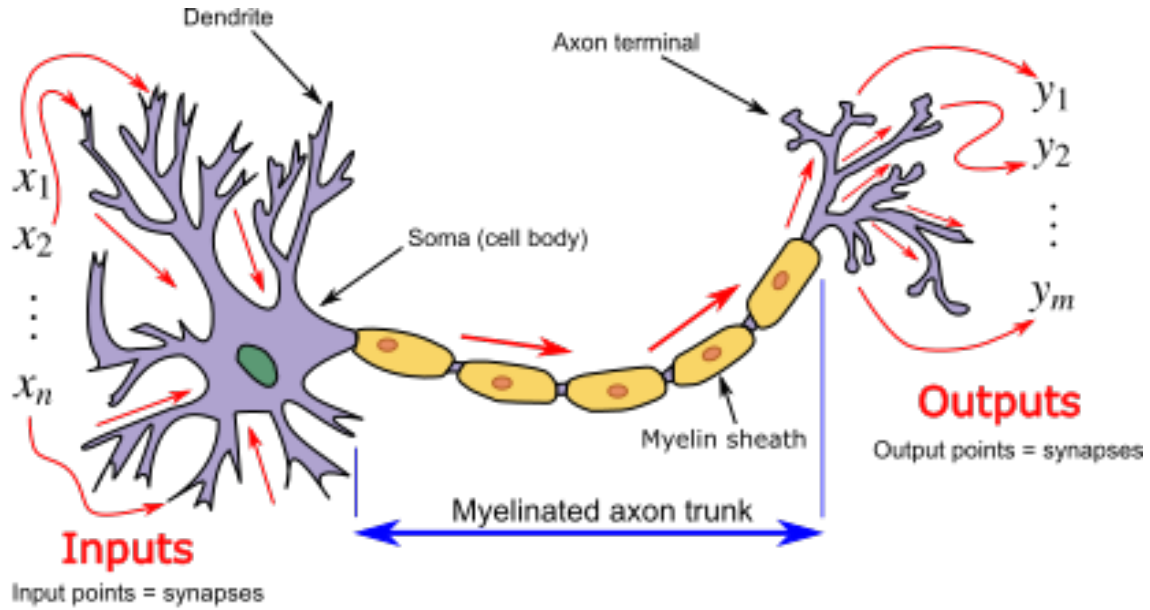
Figure 3.2: A schematic image of a biological neuron. The input signals from other neurons are received at dendrites, denoted by x_1, x_2, \dots, x_n . Processing of the signal takes place in the cell body and the outputs, y_1, y_2, \dots, y_m , are transmitted through the axon, which then acts as inputs for other neurons [93]. An artificial neuron is modeled in a similar way.
