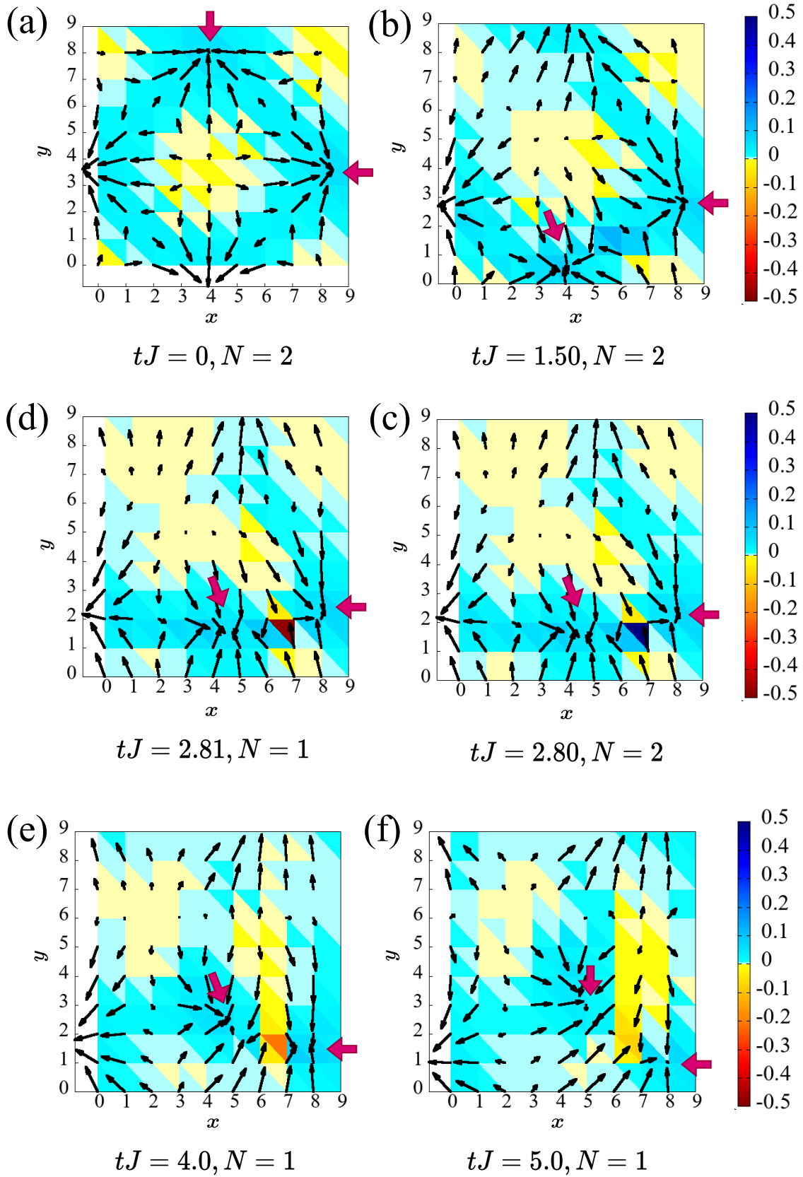
Figure 5.7: Real-time evolution of spin expectation values: snapshots of spin expectation values at different times with the skyrmion density \Omega_\Delta in the background. The quantum skyrmions (marked by arrows) move towards each other (a)-(b), interact and an exceptional configuration is formed between tJ = 2.80 and tJ = 2.81 (c)-(d), after which one quantum skyrmion decays and an elongated quantum skyrmion remains (e)-(f) [22].
