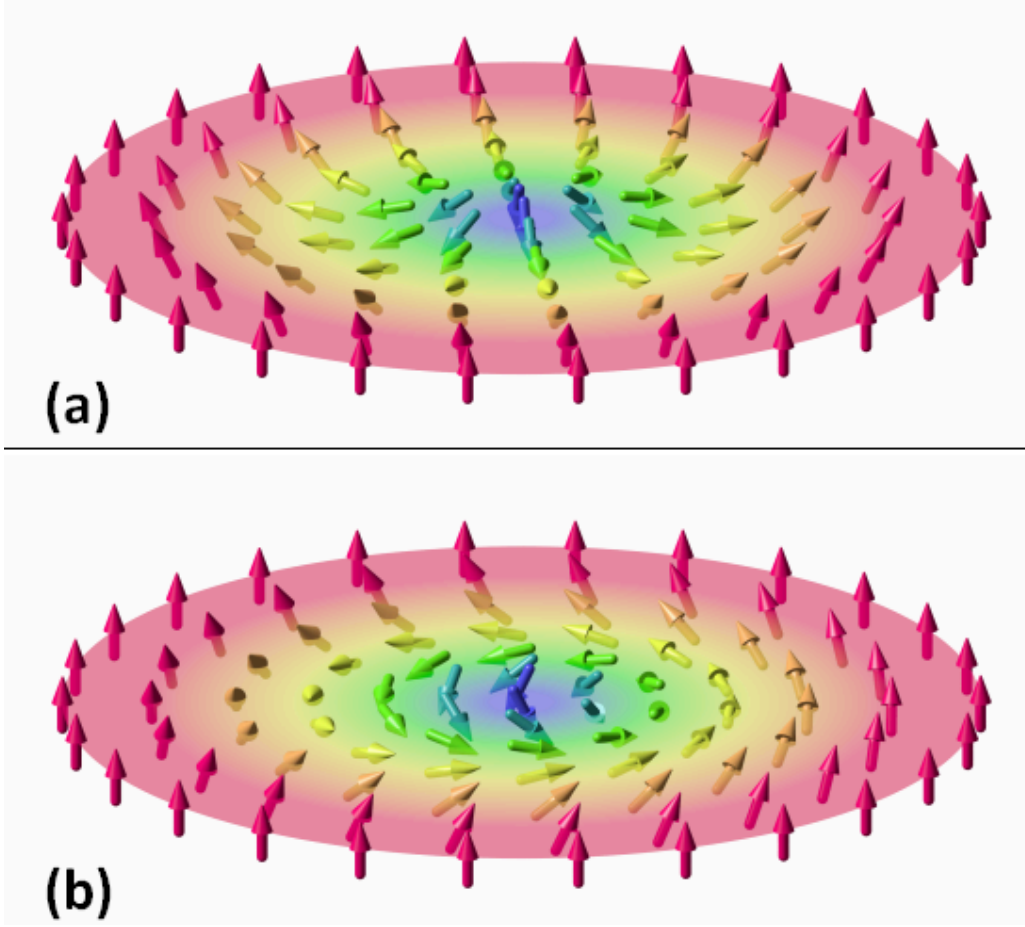
Figure 2.1: Two different types of skyrmions. (a) a Neel type skyrmion and (b) a Bloch type skyrmion [66].
