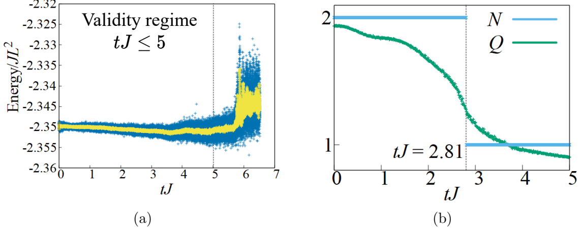
Figure 5.6: Energy and skyrmion number with time. (a) Time evolution of energy per spin of the quenched Hamiltonian in (Eq. (5.8)) over time as a quality check for the unitarity of the method. Blue shows the energy at each iteration, and yellow shows the moving average over 30 iterations. (b) Evolution of the normalized skyrmion number N and the unnormalized skyrmion number Q with time. While Q continuously decreases, N is quantized and a transition from N = 2 to N = 1 takes place at tJ = 2.81 [22].
