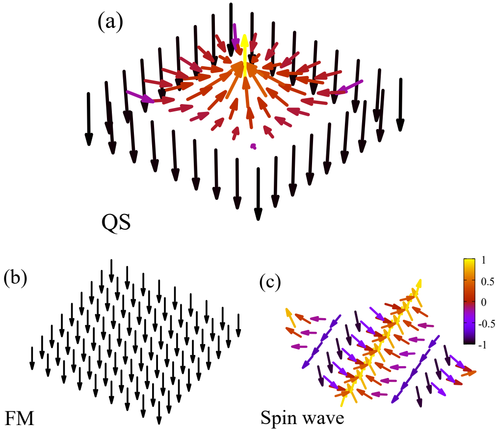
Figure 4.4: Spin expectation values of different ground states of Eq. (4.1) for a 9 \times 9 square lattice. (a) Quantum Skyrmion state (QS) at D = 0.5J, A = 0.2J and (b) Ferromagnetic state (FM) at D = 0.1J, A = J . (c) For periodic boundary conditions, we obtain a cycloidal spin spiral instead of a quantum skyrmion at D = J, A = 0.5J [21].
