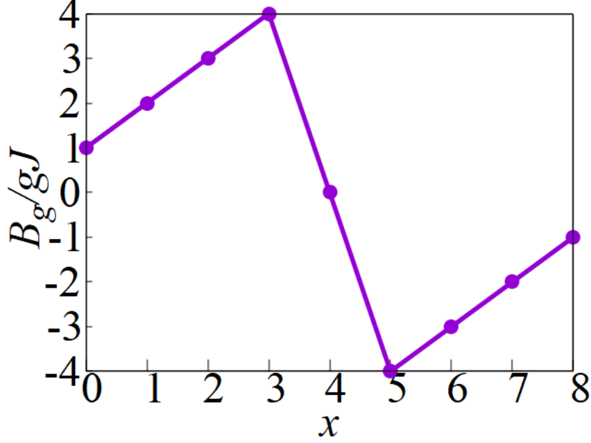
Figure 5.5: Magnetic field gradient used to move quantum skyrmions in Eq. (5.8). The magnetic field points along the z -axis and depends on the x -coordinate [22].
