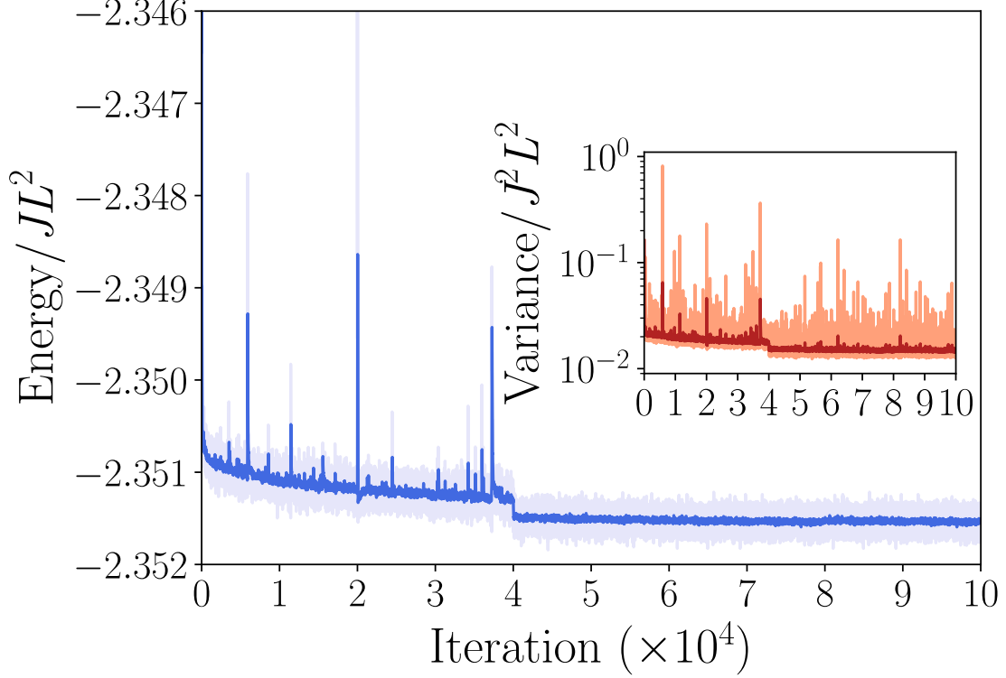
Figure 5.2: Convergence of variational energy per spin over the number of iterations for a 9 \times 9 lattice, with the energy variance per spin in the inset. The lighter color shows the values at each iteration, while the darker color shows the moving average over 30 iterations. The Hamiltonian parameters are D = J , A = 0.5J and B^z = J [22].
