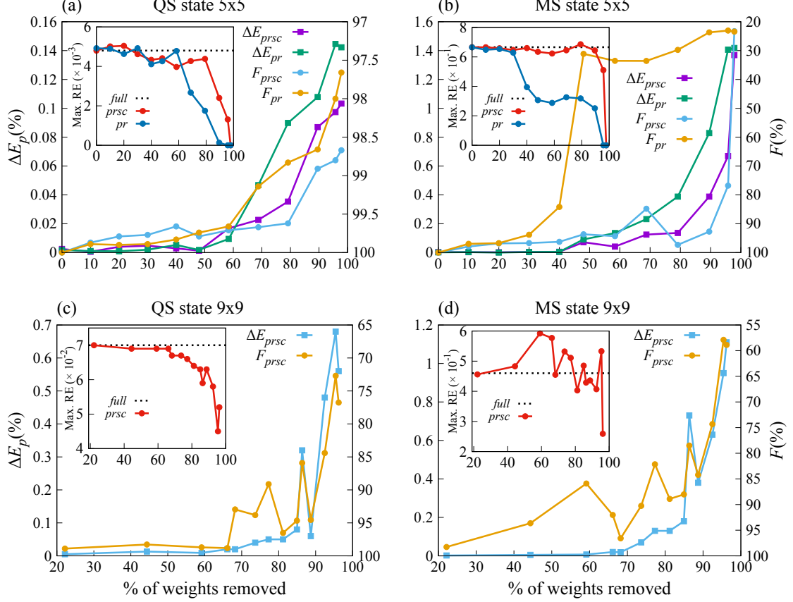
Figure 4.8: Performance metrics after pruning the neural network. \Delta E_p denotes the relative error in energy and F denotes the fidelity. pr denotes a pruned NQS trained after removing the weights from the full NQS and prsc denotes an identical network to the pr one but trained from scratch. (a) 5 \times 5 lattice QS ground state at D = J and A = 0.5J , (b) 5 \times 5 lattice MS ground state at D = 0.1J and A = 0.1J , (c) 9 \times 9 lattice QS ground state at D = 0.5J and A = 0.2J , and (d) 9 \times 9 lattice MS ground state at D = 0.1J and A = 0.1J . The inset shows the maximum values of the Renyi entropies [21].
