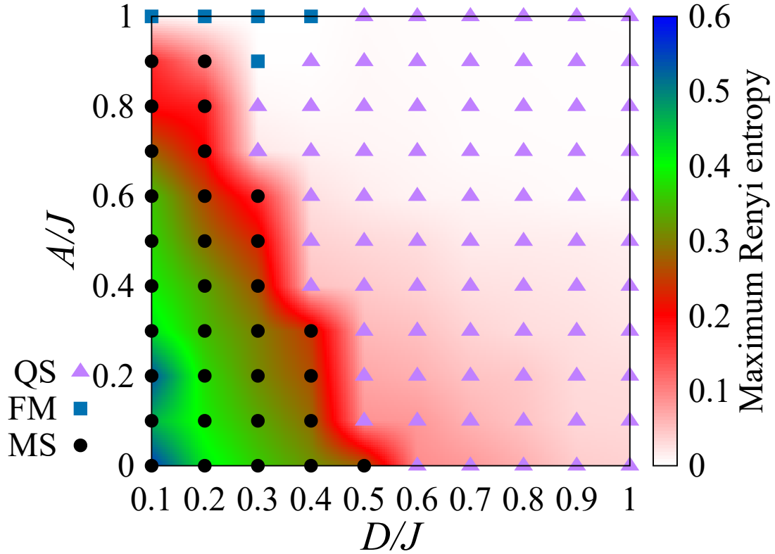
Figure 4.3: Ground state diagram for a 9 \times 9 square lattice. QS denotes the quantum skyrmion state, FM the ferromagnetic state aligned with the boundary fields, and MS the mixed state (see the main text). The color map shows the maximum Renyi entropy between two spins [21].
