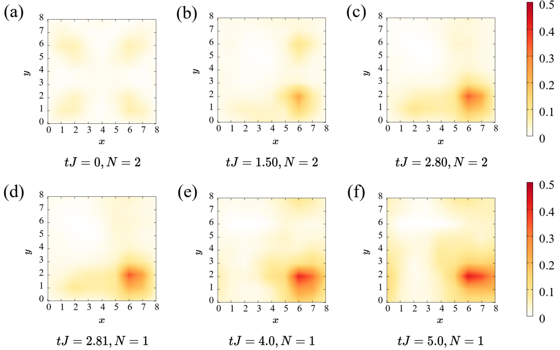
Figure 5.8: Evolution of Renyi entropy over time. The entropy increases when the quantum skyrmions interact [22].
