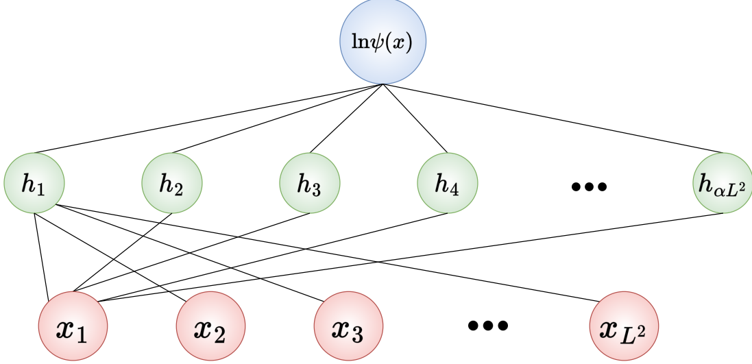
Figure 5.1: Restricted Boltzmann machine used as the neural network quantum state. The inputs are the spin configurations in \sigma^z basis, and the output is the logarithm of the wave function (Eq. (5.3)). The hidden layer contains \alpha L^2 neurons, where \alpha = 2 in our case [22].
