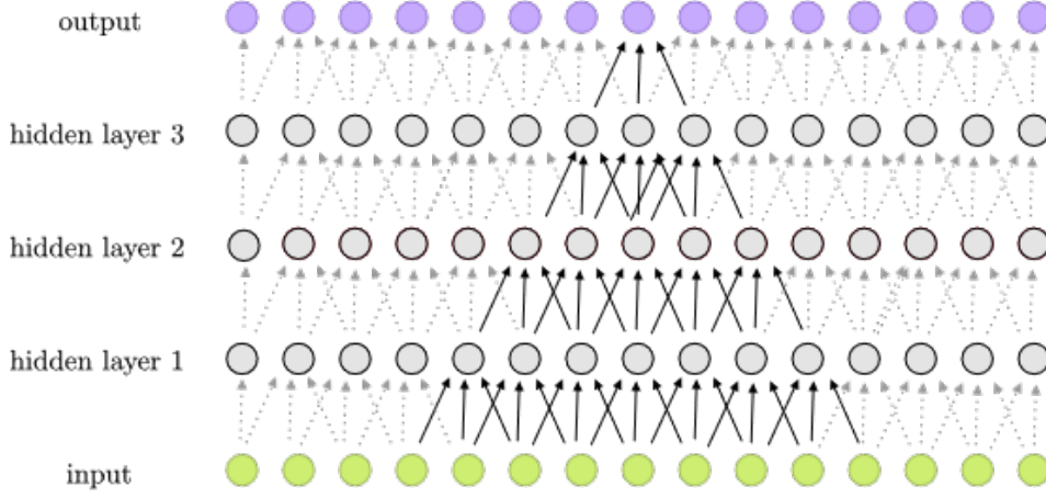
Figure 3.5: A one-dimensional, multilayered convolutional neural network (CNN). The kernel size is 3, meaning each hidden neuron takes the input from the previous 3 neurons. Unlike a fully connected neural network (Figure 3.3), the connections in a CNN are sparse and parameters are shared. This reduces the total number of parameters and the architecture is translation equivariant [103].
