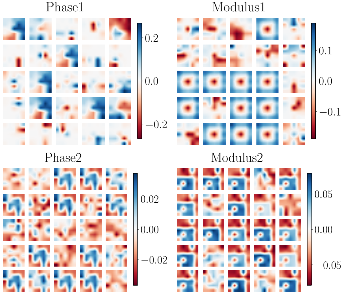
Figure 4.7: Weight distribution in the hidden layers of the quantum skyrmion ground state in a 5 \times 5 lattice at D = J and A = 0.5J . Phase1 (Phase2) and Modulus1 (Modulus2) denote the phase and modulus parts in the first (second) hidden layer, respectively. Each block shows the weights inside one hidden neuron. While the first hidden layer learns the essential features of the ground state, most of the neurons in the second hidden layer show a similar pattern [21].
