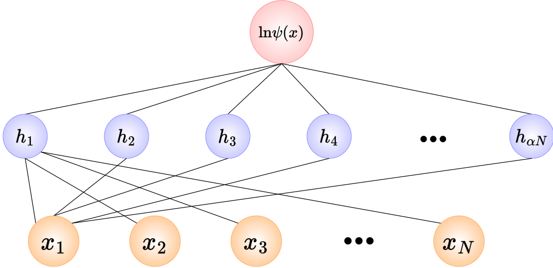
Figure 3.4: A restricted Boltzmann machine (RBM) used to represent the many-body wave function \psi(x) . The input layer consists of spin configurations. The output is the log of the wave function Eq. (3.35).
