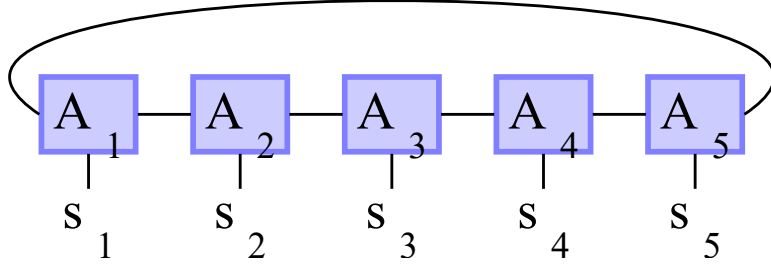
Figure 3.1: Tensor product notation of matrix product states for 5 particles [87].
