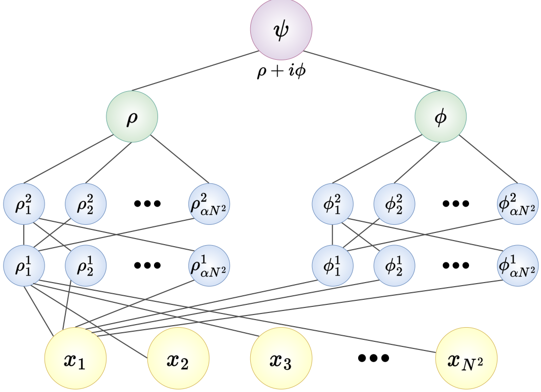
Figure 4.1: Neural network structure used as the NQS [21]. The inputs x_i are the spin configurations in the \sigma^z basis, and the output is the logarithm of the wave function. There are two fully connected networks, with two hidden layers in each, to learn the phase and the amplitude part of the wave function separately. Each hidden layer consists of \alpha N^2 neurons.
