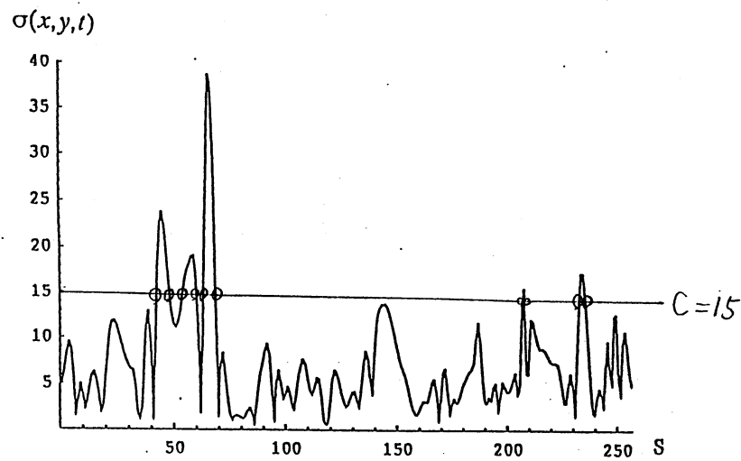
Fig.2 A horizontal slice through Fig.1. The spacings between the adjacent two points marked with circles are measured to calculate spacing distributions. The above example in the figure shows the points of the LED for the intensity c=15 .
