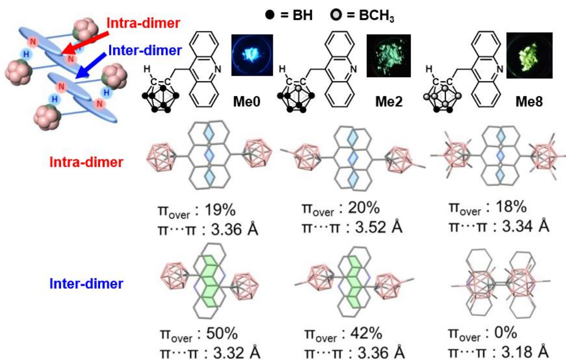
Fig. 7 Structure–property relationship between the stacking areas and color of excimer emission in the o -carborane derivatives with different number of methyl groups in the cluster unit. Reprinted with permission from ref 40. Copyright 2023 WILEY-VCH Verlag GmbH & Co. KGaA, Weinheim.
