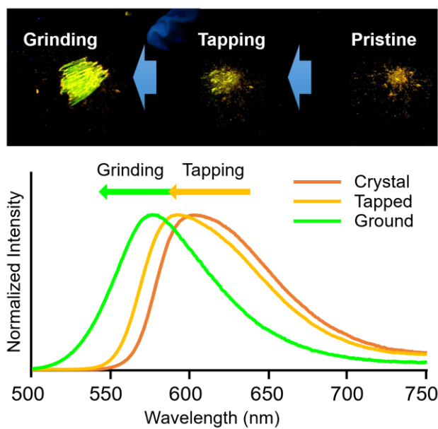
Fig. 5 Multi-step mechanochromic luminescence of 11 by tapping and subsequently grinding with the pristine crystalline sample. Adapted with permission from ref. 32.
