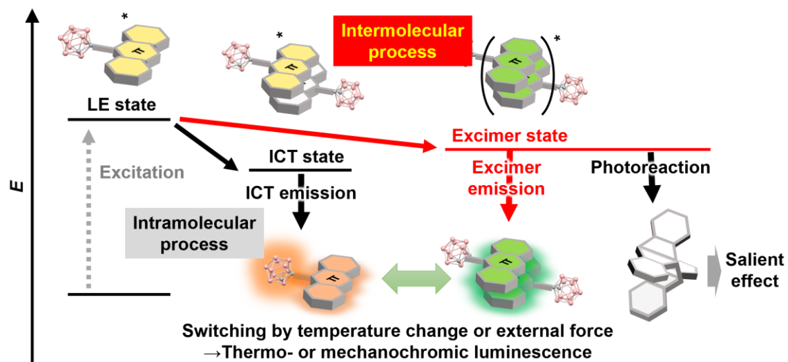
Fig. 1 Schematic illustration of stimuli-responsive luminochromic behaviors via intramolecular charge transfer (ICT) and excimer states.
