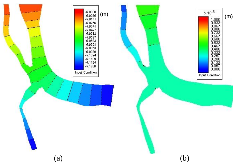
Figure 5.6 Initial bed geometry and horizontal distribution of initial mean diameter of bed material (Bank line shape: 1993), (a) Bed geometry, (b) Mean diameter of bed material
