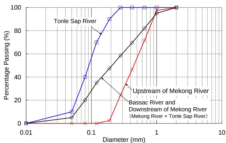
Figure 5.7 Initial size distribution of bed material
