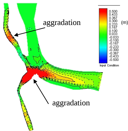
Figure 5.16 Horizontal distribution of bed deformation during dry season in Case 4
