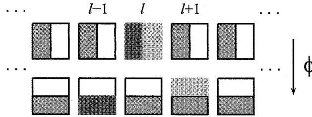
Figure 2: Schematic representation of the action of the multibaker map (2) on several cells of its phase space.
