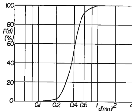
Fig. 1 The grain size accumulation curve of the sand used.
