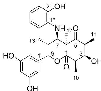
Saccharothriolide B (2)
