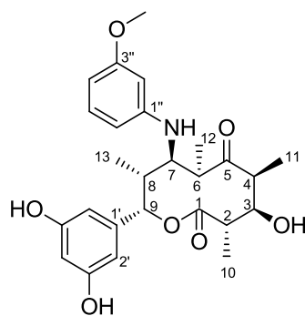
saccharothriolide J ( 13 )
