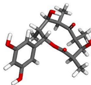
Saccharothriolide C ( 3 )
