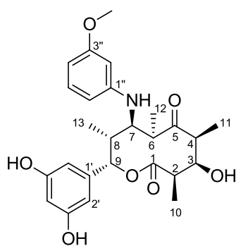
saccharothriolide I ( 12 )
