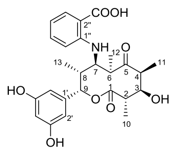
saccharothriolide D ( 4 )
