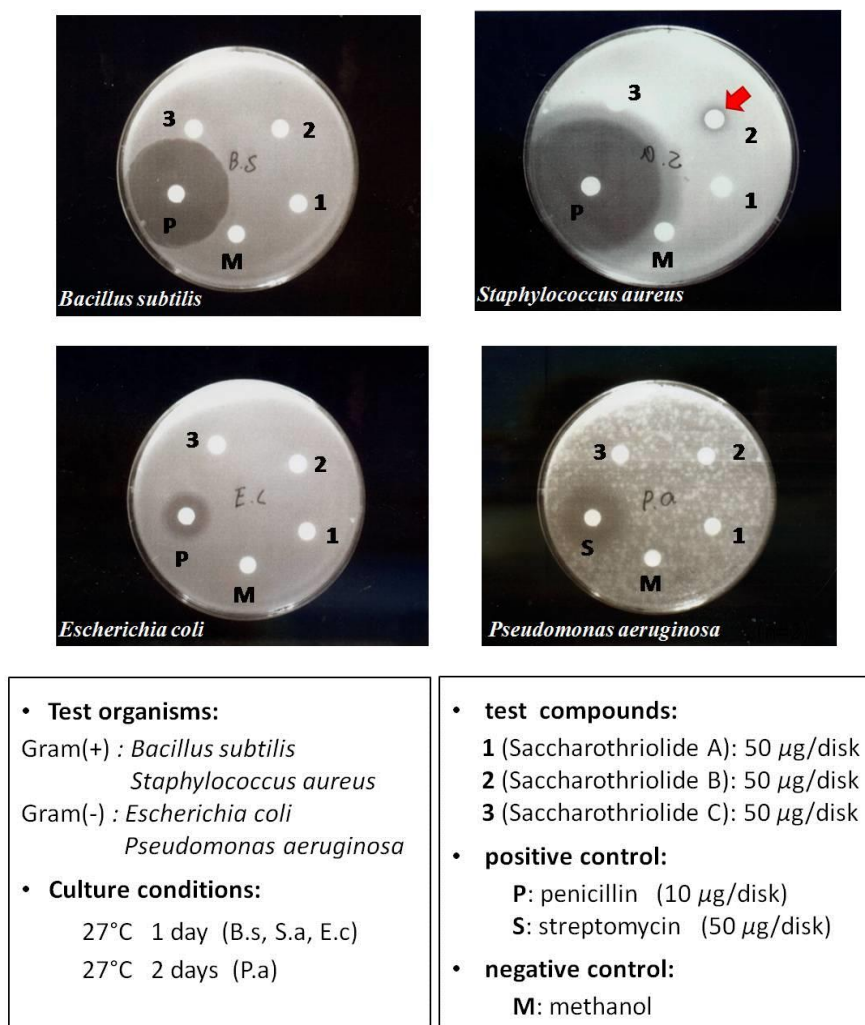
Figure 19. Antibacterial activity of saccharothriolides A-C.
