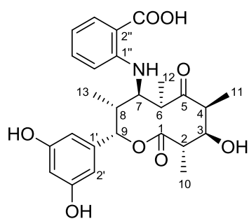
saccharothiolide D ( 4 )
