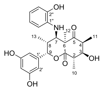
saccharothriolide E ( 5 )
