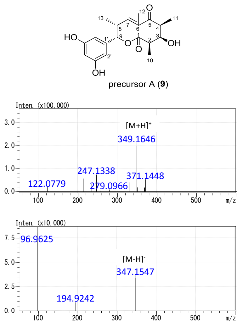
Figure S40. HR-ESI-MS spectra of precursor A ( 9 ).
