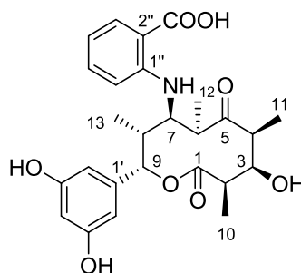
Saccharothriolide A (1)
