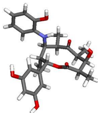
Saccharothriolide B ( 2 )
