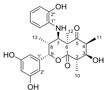
saccharothriolide E (5)
