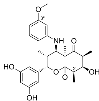
saccharothriolide I ( 12 )
