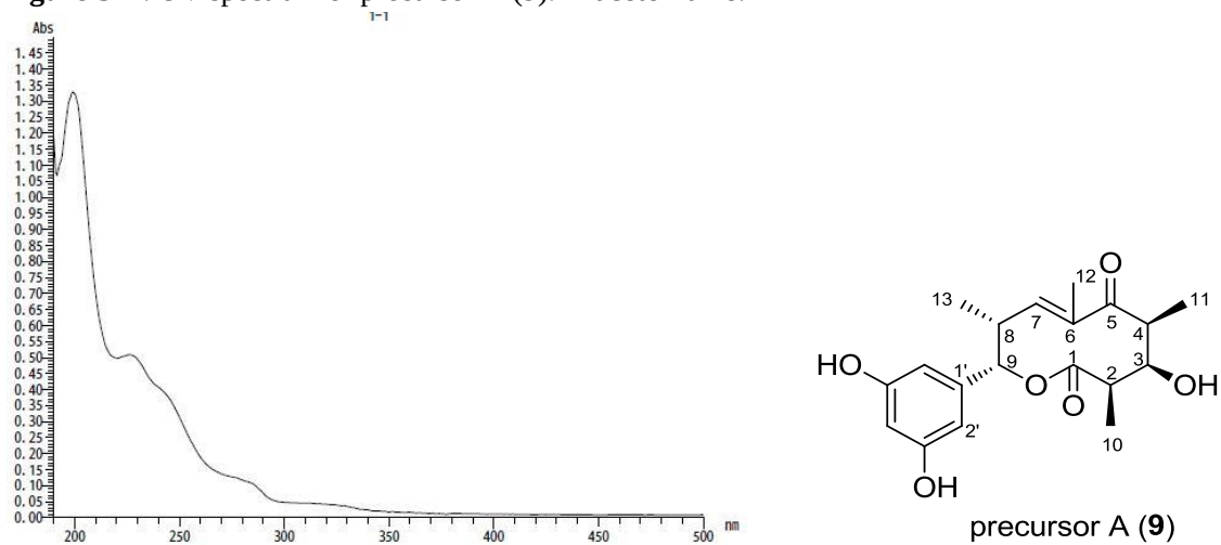
Figure S41. UV spectrum of precursor A ( 9 ), in acetonitrile.
