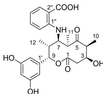
Saccharothriolide F ( 6 )
