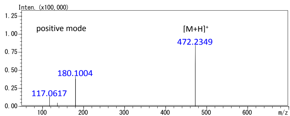
saccharothriolide J ( 13 )
