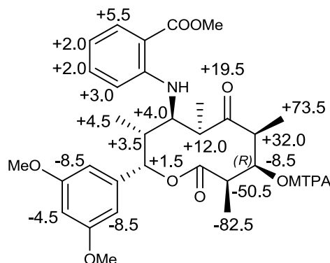
Figure 6. \Delta\delta ( \delta_S - \delta_R ) values (in Hz) for the MTPA esters of 8 .
