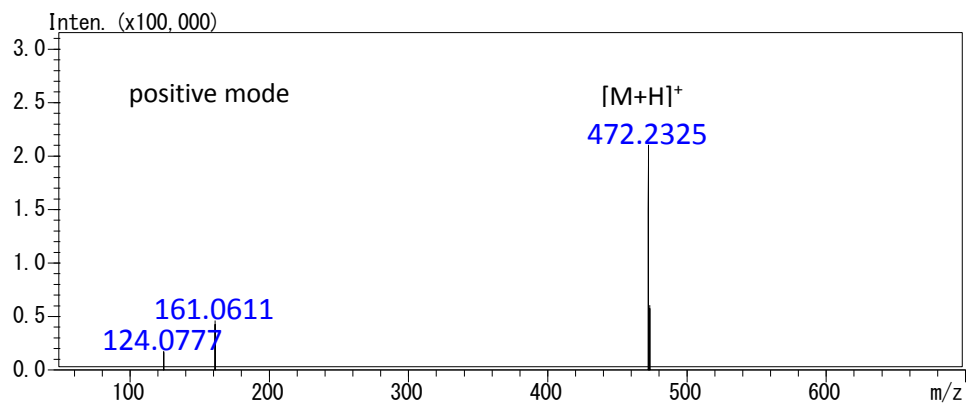
saccharothriolide H ( 11 )
