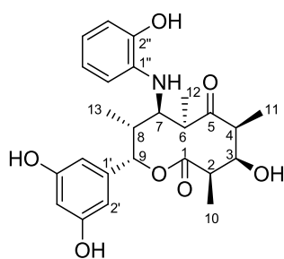
saccharothiolide B (2)
