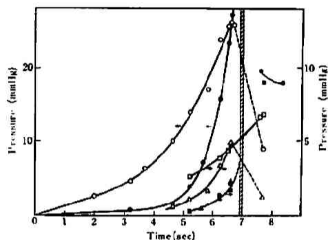
Fig. 2 Product-time curves Temperature 430°C ○: acetaldehyde, Δ: acrolein, ●: carbon monoxide, □: butadiene, ■: propylene (× 2), ▲: methane
