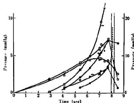
Fig. 4 Product-time curves Temperature 480°C ○: acetaldehyde, ■: acrolein, △: carbon monoxide, □: butadiene, ●: propylene (× 2), ▲: methane
