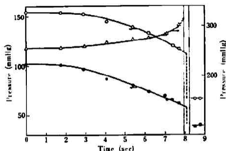
Fig. 3 Progress of the reaction Temperature 480°C ○: oxygen, ●: T2B, △: total pressure
