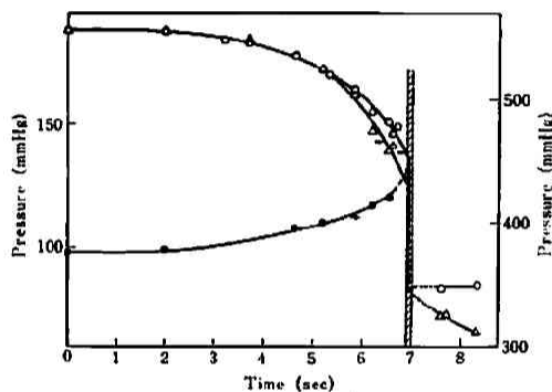
Fig. 1 Progress of the reaction Temperature 430°C Δ: oxygen, ○: T2B, ●: total pressure
