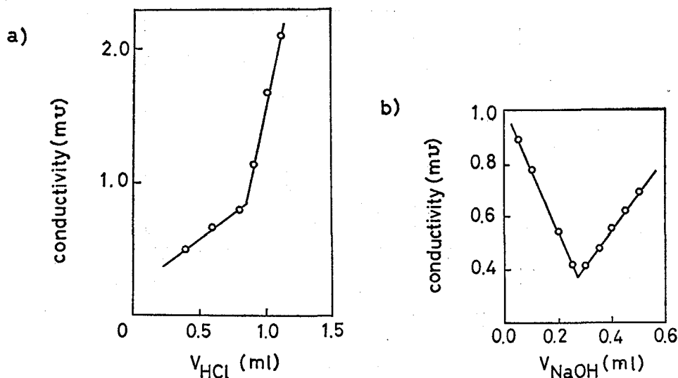
Fig. 1. Conductometric titrations of (a) PVA-AA and (b) PVA-S. Conductivity of solution is plotted against an added volume of a) acid ( V_{HCl} ) and b) alkali ( V_{NaOH} ).
