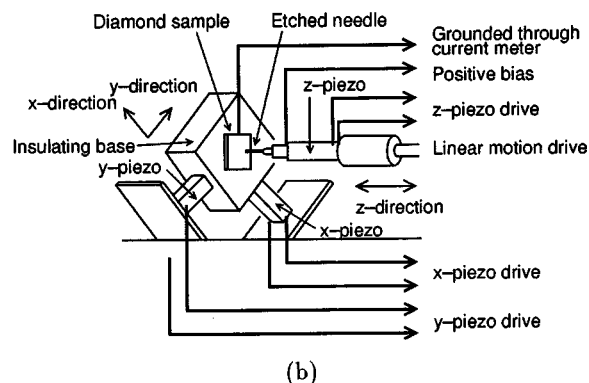
FIG. 2. Measurement system for estimation of the emission field and emission site. (a) Parallel-plate system for general measurements and field determination and (b) point measurement system for site determination.
