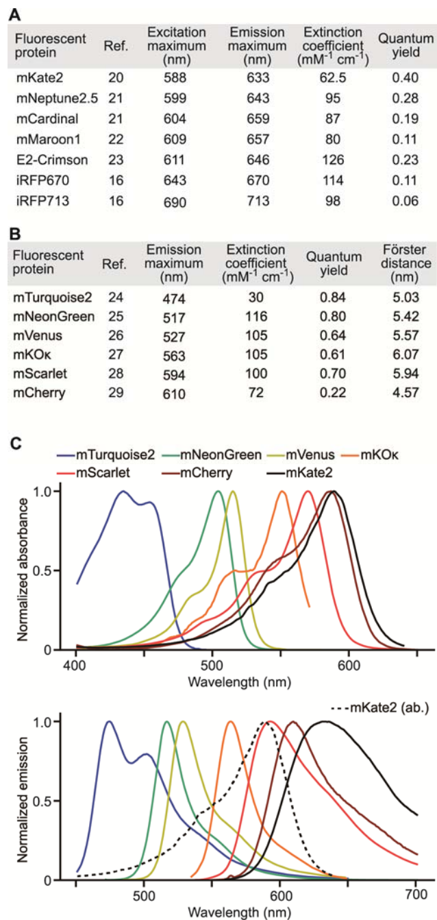
Figure S1: Properties of fluorescent proteins for the red-shifted FRET biosensor
