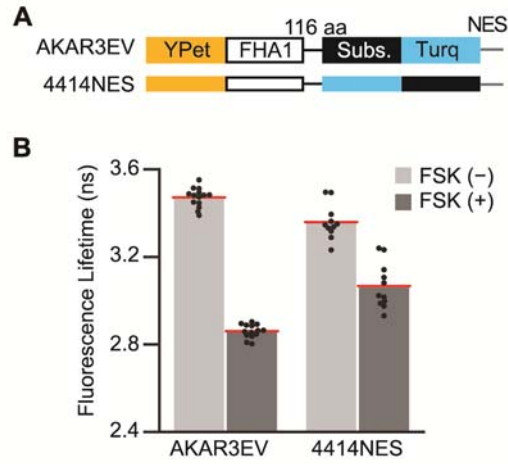
Figure S4: Application of the arrangement of Booster to the CFP/YFP pair
