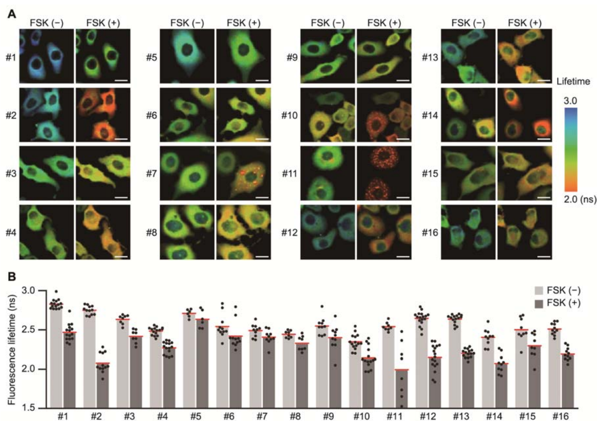
Figure S2: Optimization of the order of components
