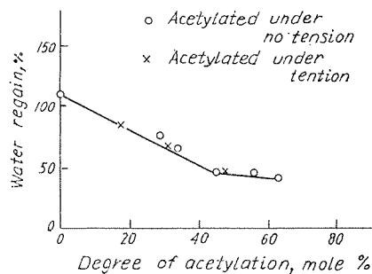
Fig. 2. Water absorption of acetylated cotton fabrics.
