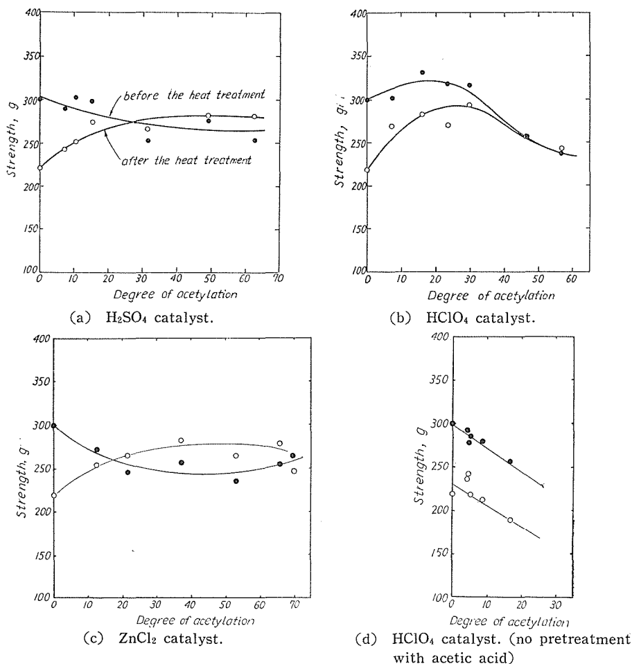
Fig. 6. The thermal stability of acetylated cotton fabrics (The change of tensile strength by heating), ● before heating; ○ after heating of 10 hours at 150°C in air. For the tensile strength measurement, 30 pieces of the warp were took out from the each fabrics and tested at RH 55~60% at room temperature. The experimental points are their averages.
