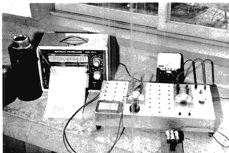
Photo 1. Experimental instruments (calorimeter, auto-recorder, bridge circuit).
