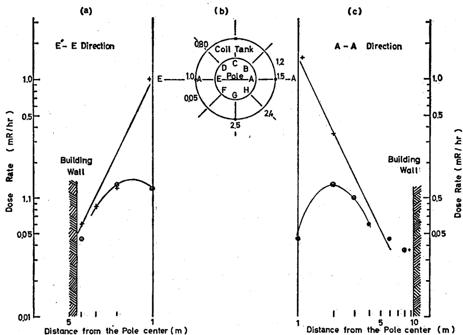
Fig. 2. Dose rate along the median plane between the two poles on the 13 th of March 1971. The numbers denote the dose rate in mR/hr.
