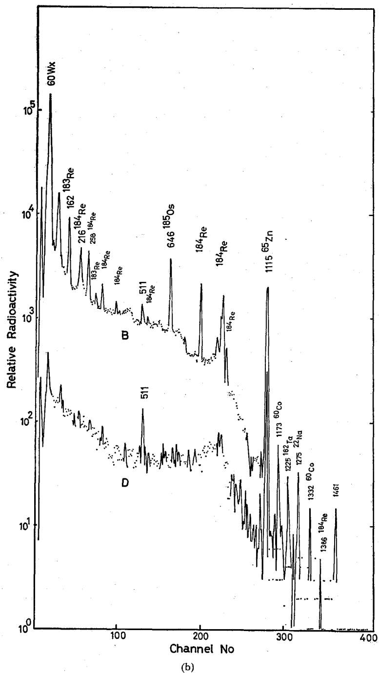
Fig. 4. \gamma -ray spectrum of the sample smeared out from several portions of the deflector electrode.
