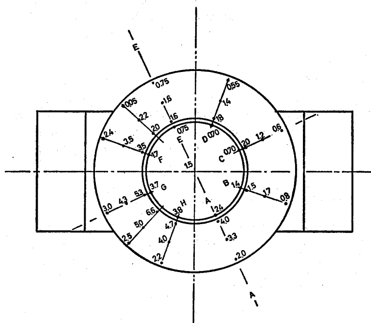
Fig. 1. Dose rate at the surface of the pole and of the coil tank on the 21 st of April 1971. The numbers denote the dose rate in mR/hr unit.
