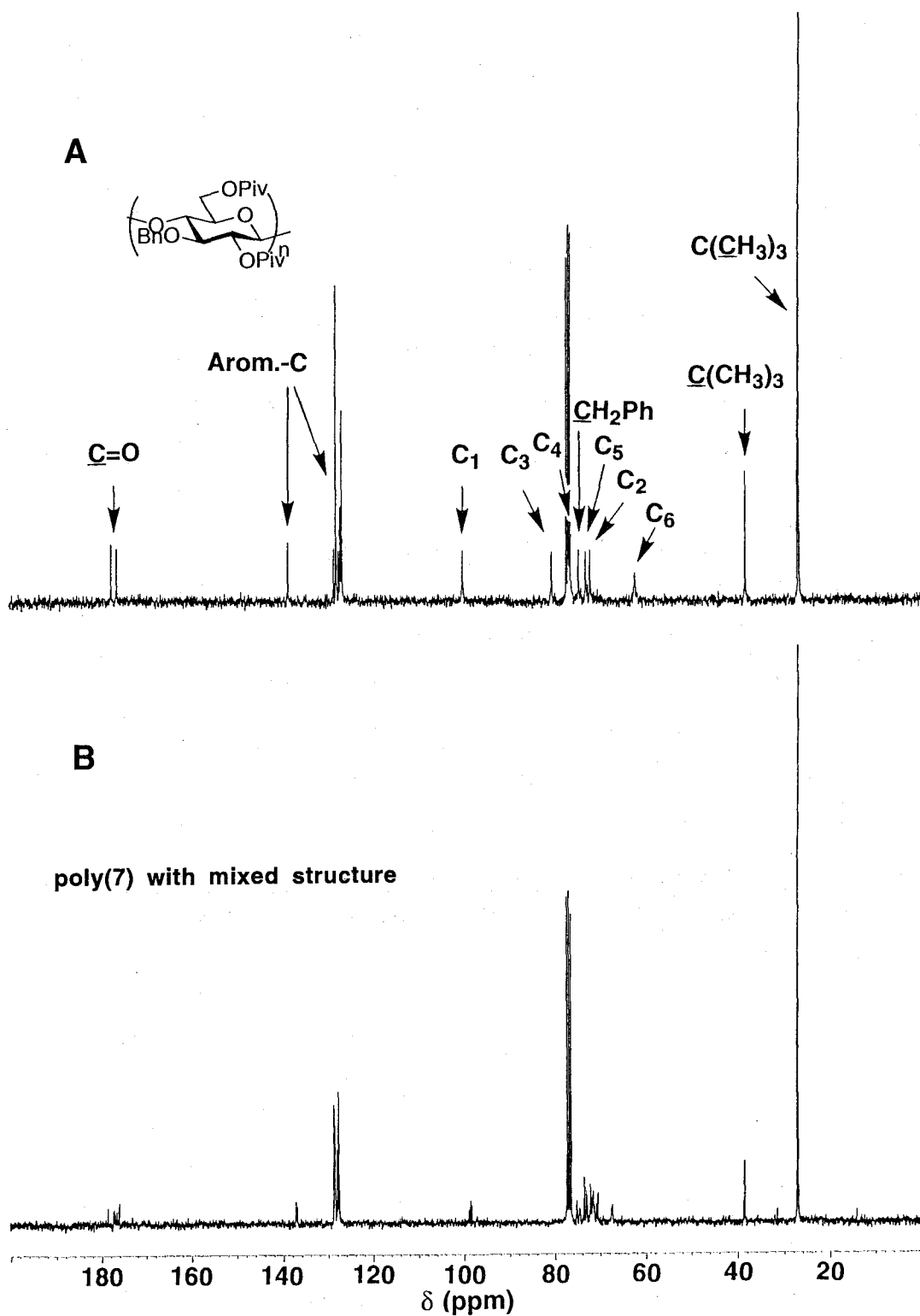
Figure 11. 75-MHz ^{13}\text{C} -NMR spectra of (A) poly(6) polymerized at 0^\circ\text{C} (Table 10, experiment no. 5), and (B) poly(7) polymerized at -30^\circ\text{C} (Table 10, experiment no. 7) ( \text{CDCl}_3 as solvent).
