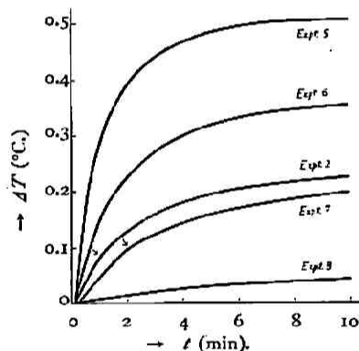
Fig. 5.—Influence of dilution.
