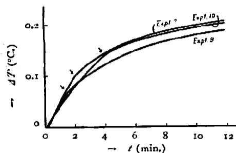
Fig. 8.—Salt effect.
