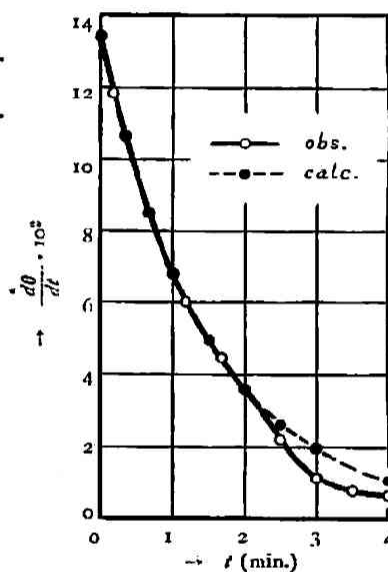
Fig. 12.—Expt. 12 (Pseudo-unimolecular).
