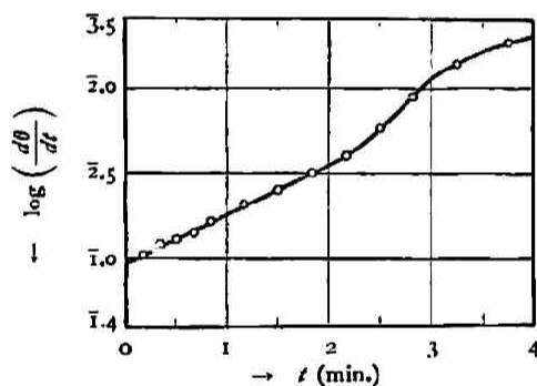
Fig. 11.—Expt. 12 (Pseudo-unimolecular).
