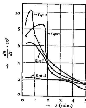
Fig. 16.—Variation of [KIO_3] .
