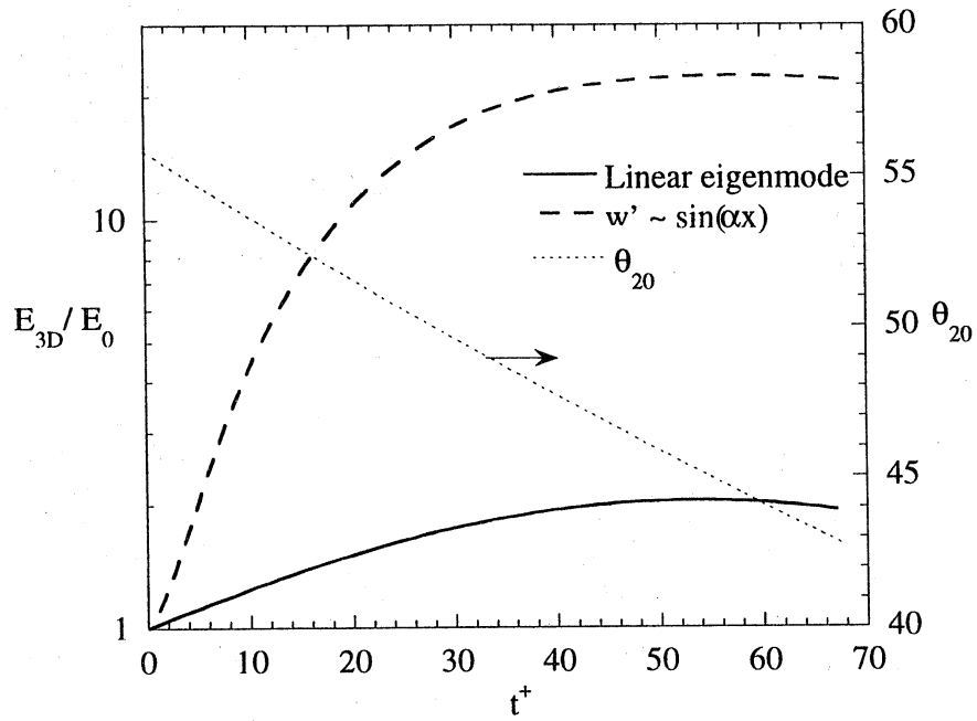
Figure 6. Evolution of 3D energy (all x-dependent modes), for most unstable linear eigenmode (solid) and w(x) linear transient disturbance (dashed). The viscous streak annihilation is reflected by the decreasing streak vortex line lift angle (dotted).
