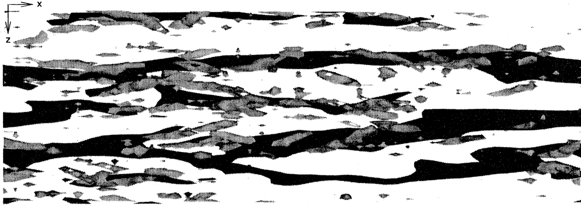
Figure 1. Lifted low-speed streaks (black) illustrated by u' < 0 at y^+ = 20 and streamwise vortices (grey) indicated by the Jeong & Hussain (1995) vortex definition in the region 0 < y^+ < 60 .
