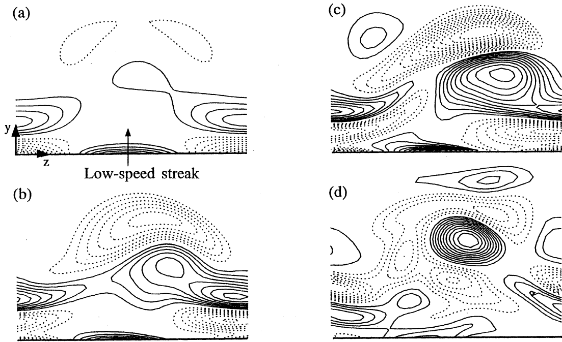
Figure 8. Streamwise vortex formation due to finite-amplitude streak instability, illustrated by cross-stream distributions of \omega_x at (a) t^+ = 17 , (b) t^+ = 51 , (c) t^+ = 103 , (d) t^+ = 928 . Planes in (b) and (c) are tracked with the instability phase speed of approximately 0.6U_c .
