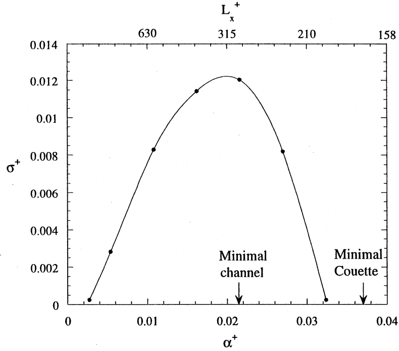
Figure 3. Growth rate of most-unstable sinuous mode versus streamwise wavenumber, for streak distribution in figure 1 with \omega_y^+|_{\max}=0.35 , corresponding to a streak lift angle of \theta_{20}=56^\circ .
