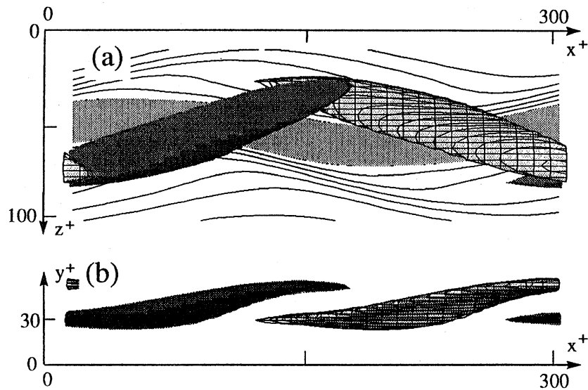
Figure 9. Streamwise vortices' (x, z) plane tilting, x -overlapping, and location relative to a low-speed streak in (a) top view, (b) side view. The 80% isosurfaces of +\omega_x and -\omega_x at t^+ = 103 are (dark) shaded and hatched respectively; contours of u at y^+ = 20 are overlaid in (a), with low levels of u light-shaded to demarcate the low-speed streak.
