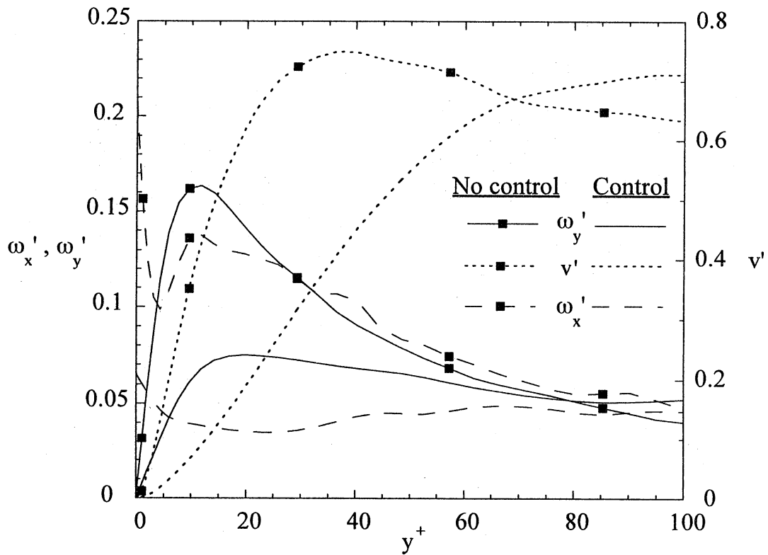
Figure 13. Suppression of v' , \omega_x' , and \omega_y' by large-scale control at t_0^+=500 , with Re=1800 and frozen 6% forcing.
