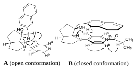
Figure 1. 1 H NMR study of 1 (A) and its acyliminium ion (B) in CDCl 3 at 20 °C. Arrows denote the observed NOE's. In A, protons H a , H b and H c , H d appear at δ 8.01 and 6.37 ppm, respectively. In B, protons H a , H b , H c , and H d appear independently at δ 7.45, 8.73, 5.69, and 6.87 ppm, respectively.
