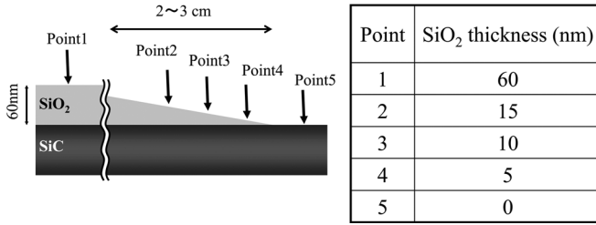
FIG. 1. Schematic diagram of the points measured by XPS with gradient etching.
