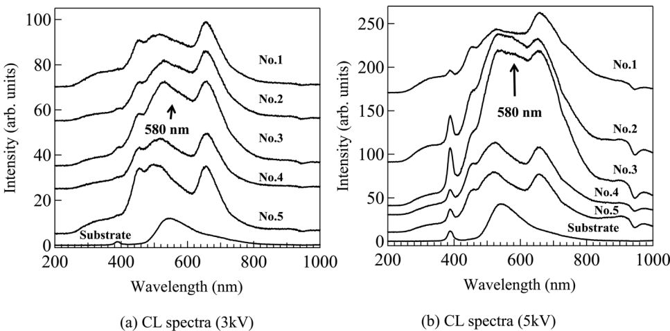
FIG. 2. CL spectra of \text{SiO}_2 films on 4H-SiC substrate measured at acceleration voltages of (a) 3 kV and (b) 5 kV.
