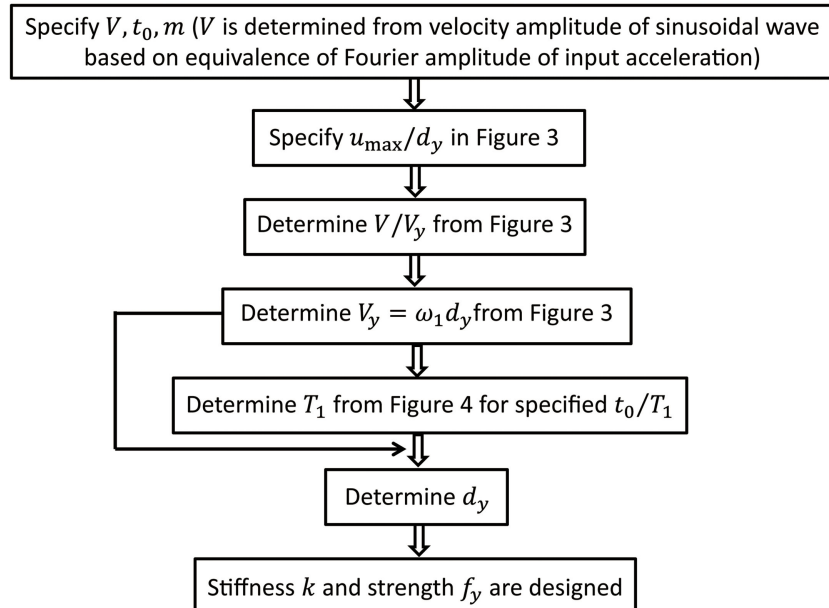
FIGURE 11 | Flowchart for design of stiffness and strength.
