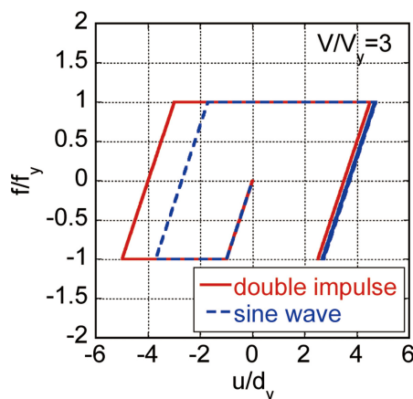
FIGURE 10 | Comparison of restoring-force characteristic under double impulse and that under the corresponding one-cycle sinusoidal wave.
