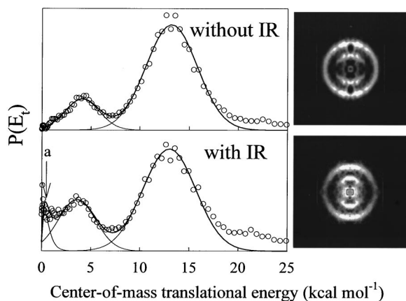
FIG. 6. Equatorial slices of the 3D images and P(E_t) for S(1D) observed from OCS photodissociation at 230.00 nm. The double rings correspond to the bimodal rotational energy distributions of CO. Upper panel was measured with UV (0.2 mJ/pulse) and without IR laser pulse. Lower panel was measured with increasing UV laser intensity (0.5 mJ/pulse) and with IR (80 mJ/pulse). A peak marked with (a) is due to IR multiphoton dissociation, which corresponds to the central peak of the lower image.
