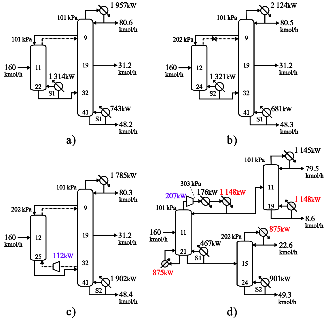
Figure 3.10. Optimal distillation sequences obtain from rigorous simulations:
