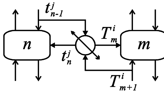
Figure 2.9. Detailed representation of energy transfer between stages.
