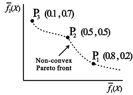
Figure 4.7. Representation of a non-convex Pareto front
