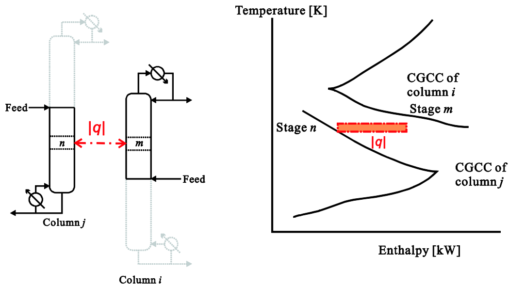
Figure 2.4. Internal heat integration between two columns (left) and its CGCC representation in an Enthalpy-Temperature diagram (right)
