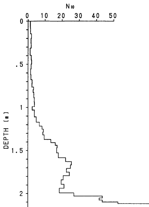
Fig. 4. An example of the vertical change in cone penetration resistance N_{10} obtained at the site B3.
