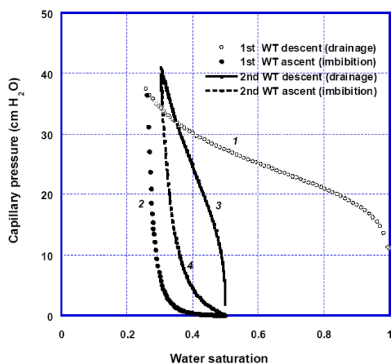
Fig. 6. Fitted S - p relation under the influence of water table fluctuation
