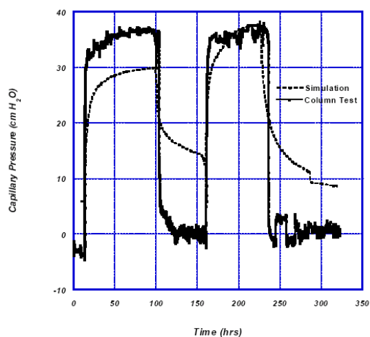
Fig. 10. Simulated and measured capillary pressure
