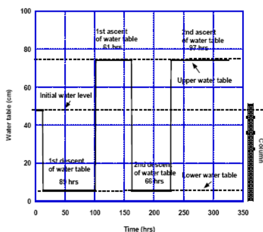
Fig. 3 Variation of the water tank position
