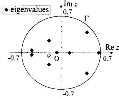
Figure 1: Computed eigenvalues for the n = 1000 and \epsilon = 0.01 case.
