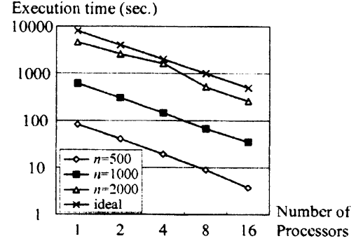
Figure 2: Execution time of our algorithm on Fujitsu HPC2500.
