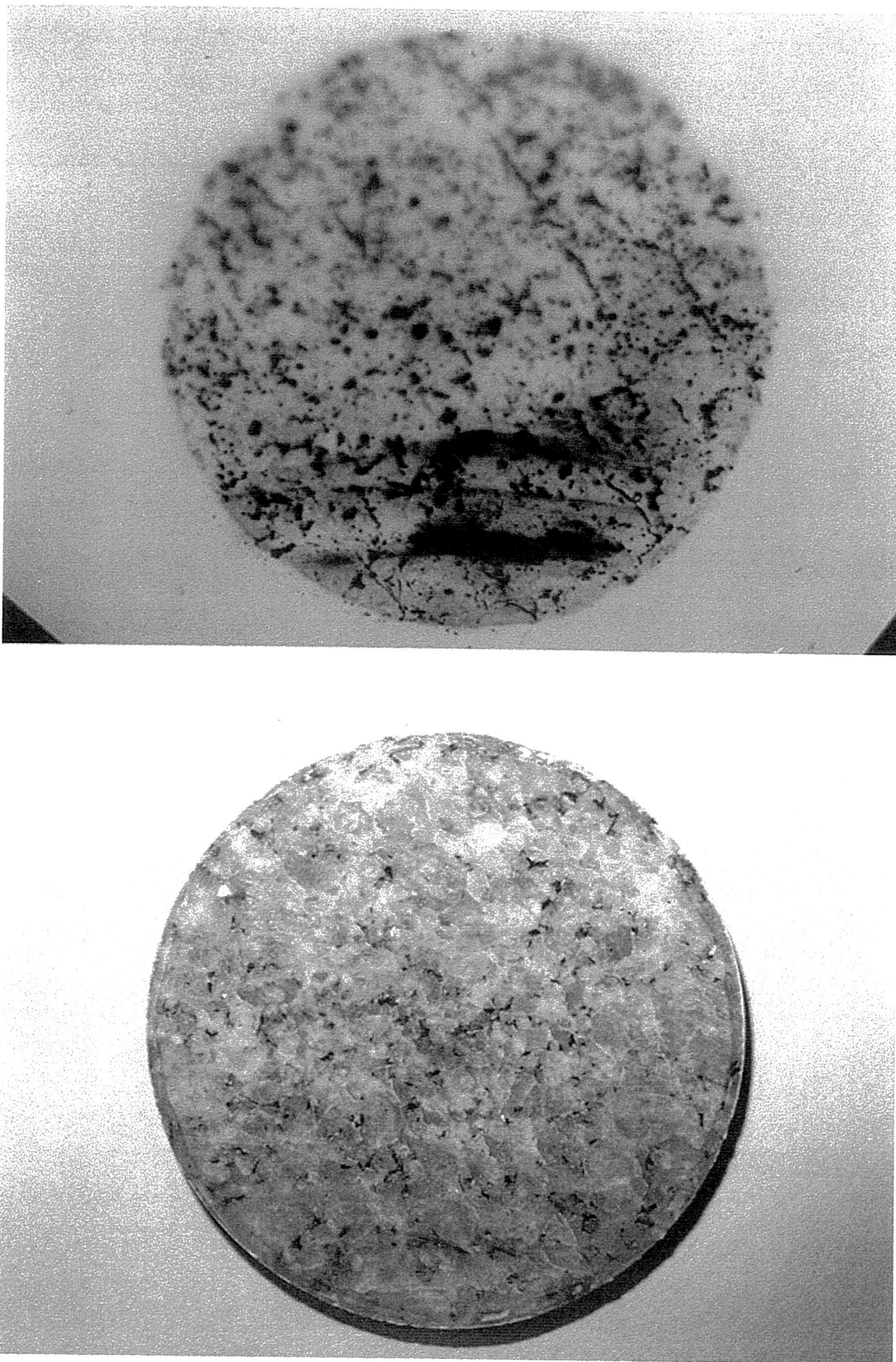
Fig. 7-2c Autoradiographic and optical images for the "hot" side of the granite disk, F9 used in the 1 st series of diffusion experiment for actinide carbonate complexes.
