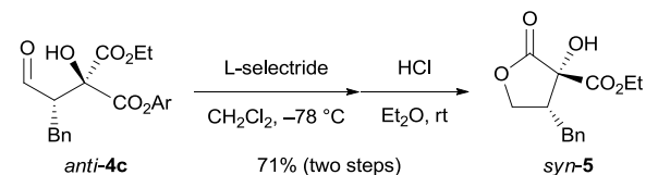
Scheme 1 Synthesis of α-hydroxy-γ-lactone syn - 5 .
