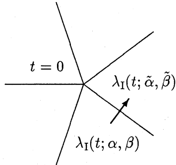
Figure 3: Stokes curves of (P_I) .
