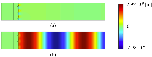
FIG. 6. Elastic medium in the optimal configuration: (a) distribution of displacement u along the x -axis and (b) distribution of displacement v along the y -axis.
