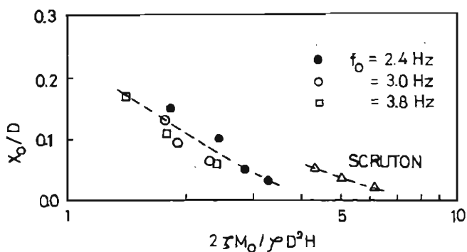
Fig. 4 Damping-Maximum Amplitude Relation. The abscissa is \zeta M_0 / \rho D^2 H for Scruton's data.
