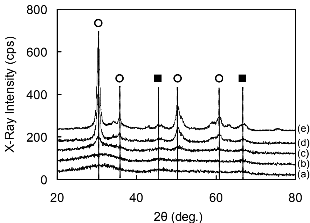
Fig. 2. XRD patterns of AZT at various calcination temperatures. (a) AZT773, (b) AZT873, (c) AZT973, (d) AZT1073, (e) AZT1173. \circ : tetragonal \text{ZrO}_2 and \blacksquare : \gamma\text{-Al}_2\text{O}_3 .
