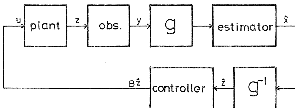
Fig. 6 Block diagram.
