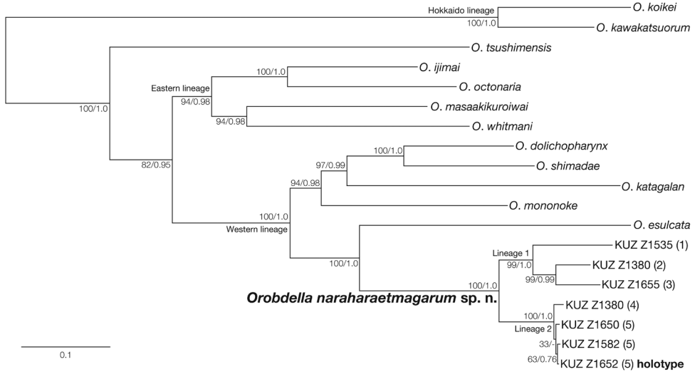
Figure 7. Maximum likelihood tree (ln L = -15057.02 ) for 3,008 bp of mitochondrial COI, tRNA Cys , tRNA Met , 12S rRNA, tRNA Val , 16S rRNA, tRNA Leu and ND1 markers. Numbers on nodes represent bootstrap values for maximum likelihood and Bayesian posterior probabilities.
