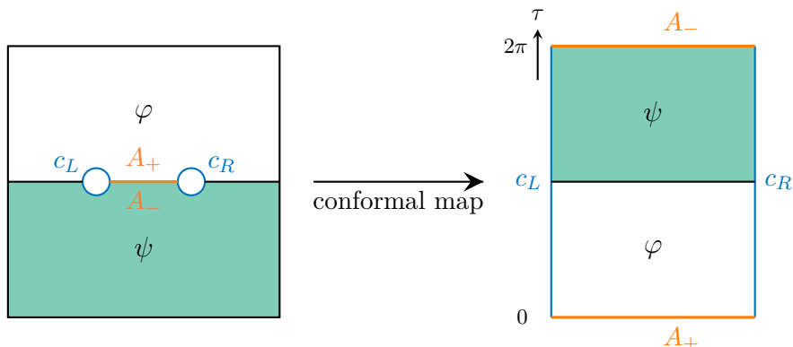
Figure 15. The pseudo entropy for an interval in CFT 2 [Left] and the conformal transformation to the cylinder [Right].
