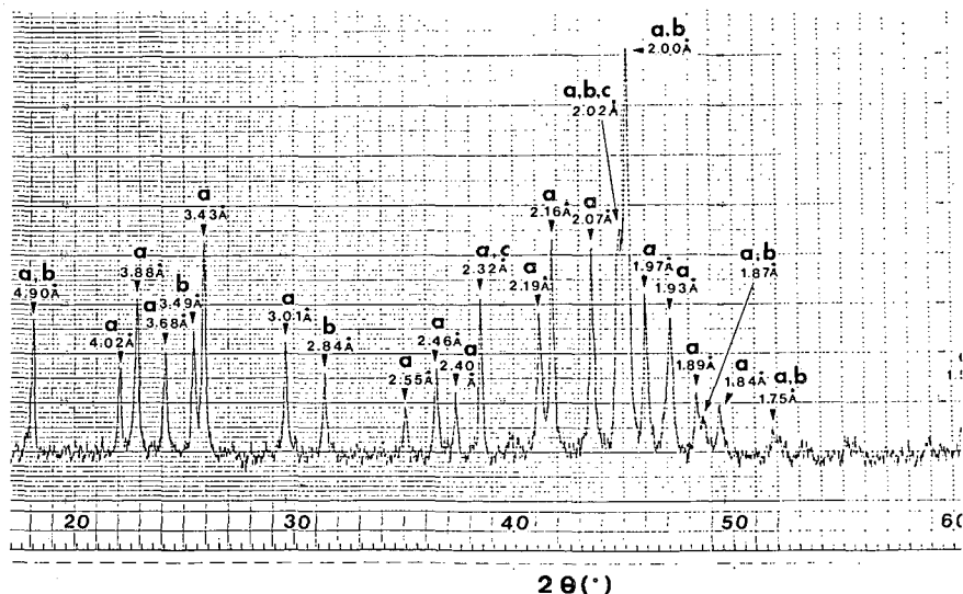
Fig. 1. X-ray diffraction pattern of 42% Ni-Al powder alloy. a, b and c denote the diffraction lines from \text{NiAl}_3 , \text{Ni}_2\text{Al}_3 and Al respectively.
