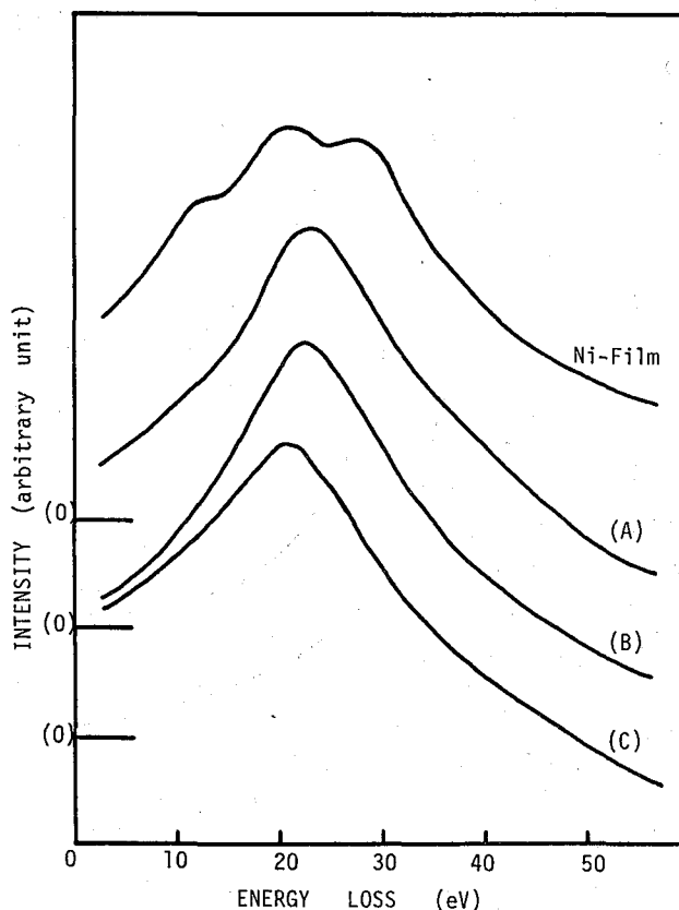
Fig. 8. The plasmon loss spectrum of Raney nickel catalyst developed in 5%(A), 20%(B) NaOH solutions and in glycol acid after treated in 5% NaOH solution(C). The spectra of Ni-film is also exhibited for comparison.
