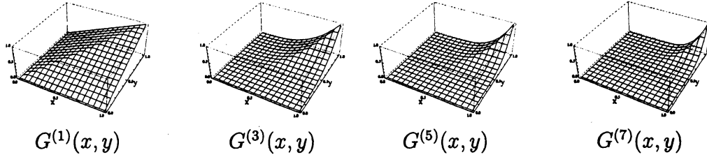
図 1 G^{(p)}(x, y), p = 1, 3, 5, 7
