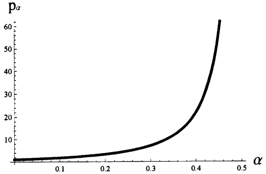
図3 p_\alpha = \frac{\log(\frac{1}{2}-\alpha)}{\log(\frac{1}{2}+\alpha)}, \alpha \in ]0, \frac{1}{2}[
