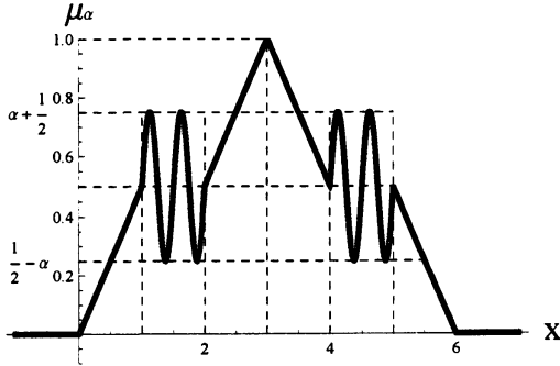
図2 \mu_\alpha(x), \alpha \in [0, \frac{1}{2}[
