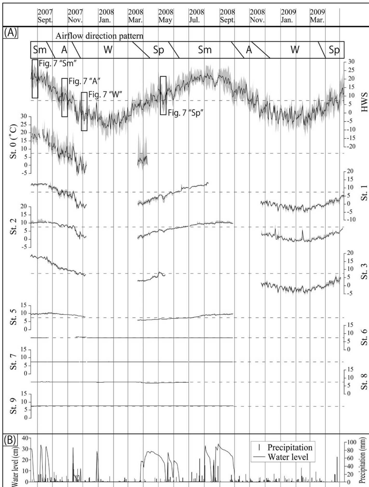
Figure 5: Monitoring results for temperature and water level of the underground river. (A) Air temperature (°C) and airflow "season". Station locations are indicated in Figure 3. Airflow "season" depends upon whether or not the outside air temperature (OAT) is higher than the inner air temperature (IAT=7.5°C). Sp: OAT MAX < IAT=7.5°C < OAT min; Sm: IAT=7.5°C < OAT min < OAT MAX; A: OAT min < IAT=7.5°C < OAT MAX; W: OAT min < OAT MAX < IAT=7.5°C. Sections within the black rectangles within the HWS (Hokuto Weather Station) data are enlarged in Figure 7 to illustrate a typical "term" within each seasonal division. However air temperatures of Stations 0, 1, 2, 3, 5 are fluctuating, that of Stations 6, 7, 8, 9 are stable. (B): Flow rate of the underground river. Each of the peaks corresponds to a significant discharge event; the underground river normally flows only when precipitation exceeds 40mm/day.
