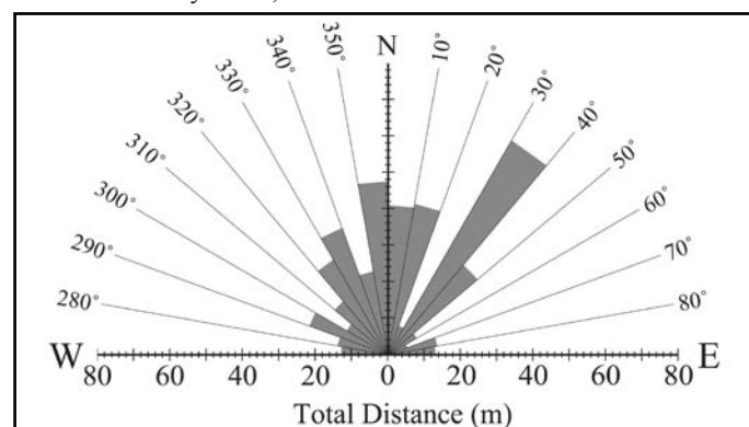
Figure 4: Passage direction variation in Hokkai Cave. The dominant directions are NE-SW ( 30^\circ – 50^\circ ), NNW-SSE ( 320^\circ – 340^\circ ) and N-S ( 350^\circ – 20^\circ ).
