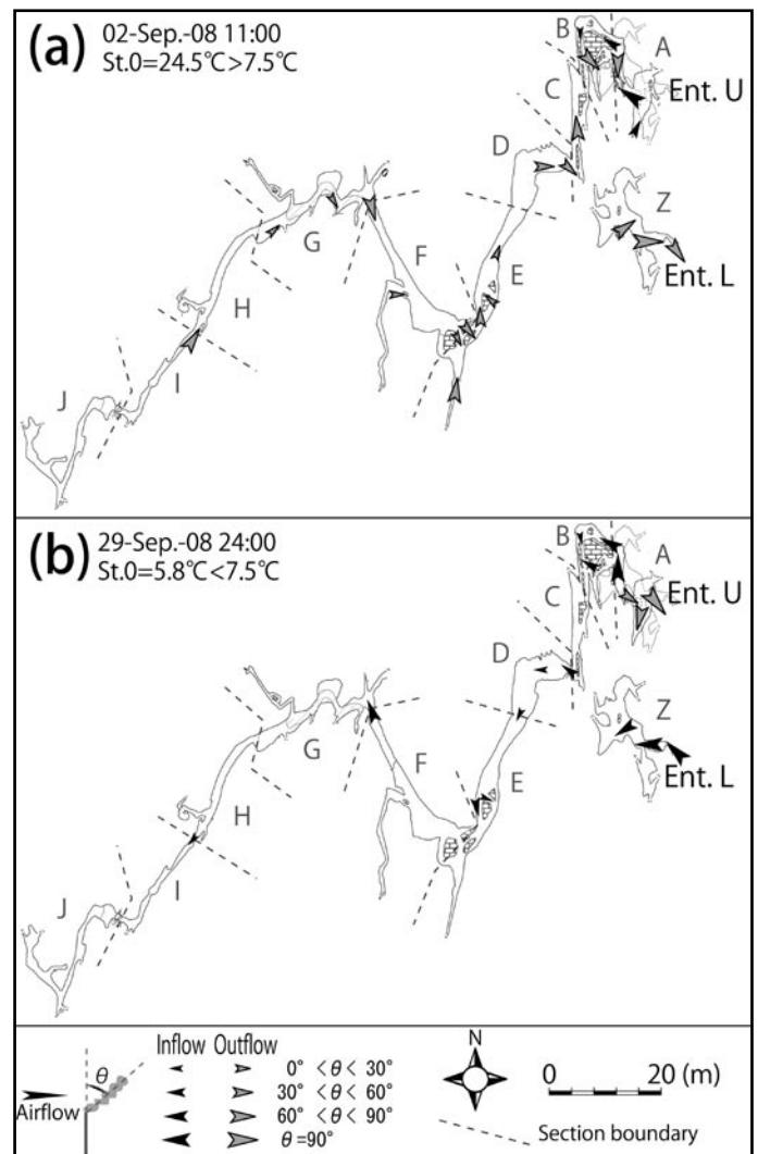
Figure 6: Airflow direction and intensity in Hokkai Cave. Airflow direction depends on whether the outside air temperature (OAT) is higher than the inner air temperature (IAT) (about 7.5°C = annual mean air temperature) or not. (a) When the OAT is higher than the IAT, air flows from upper to lower and from inner to outer. (b) When the OAT is lower than the IAT, air flows from lower to upper and from outer to inner.
